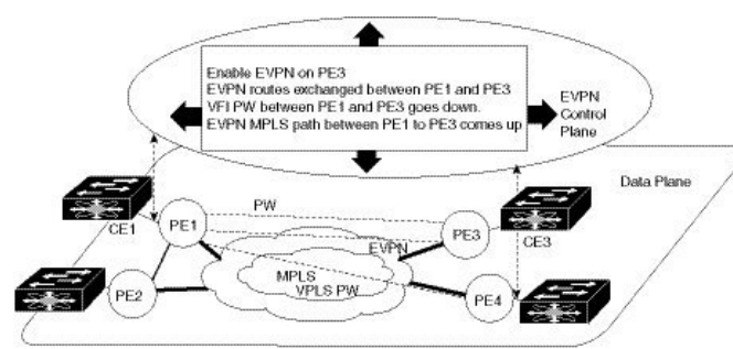
Figure 48: EVPN MPLS Seamless Integration with VPLS
