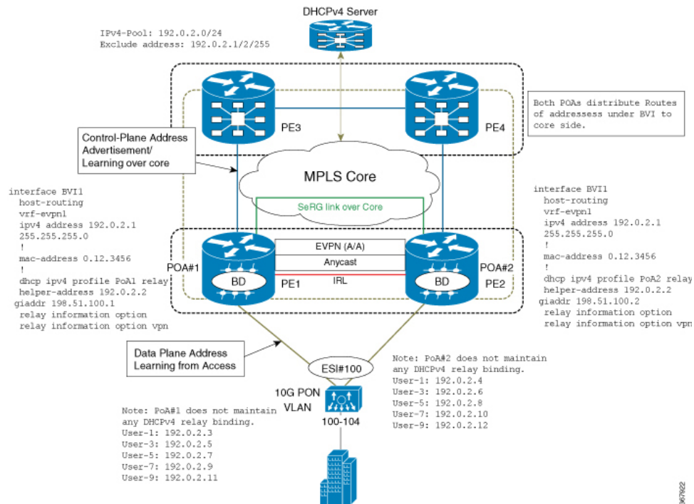
Figure 69: DHCPv4 Relay Handling for EVPN and DHCPv4 Server in Different VRF
