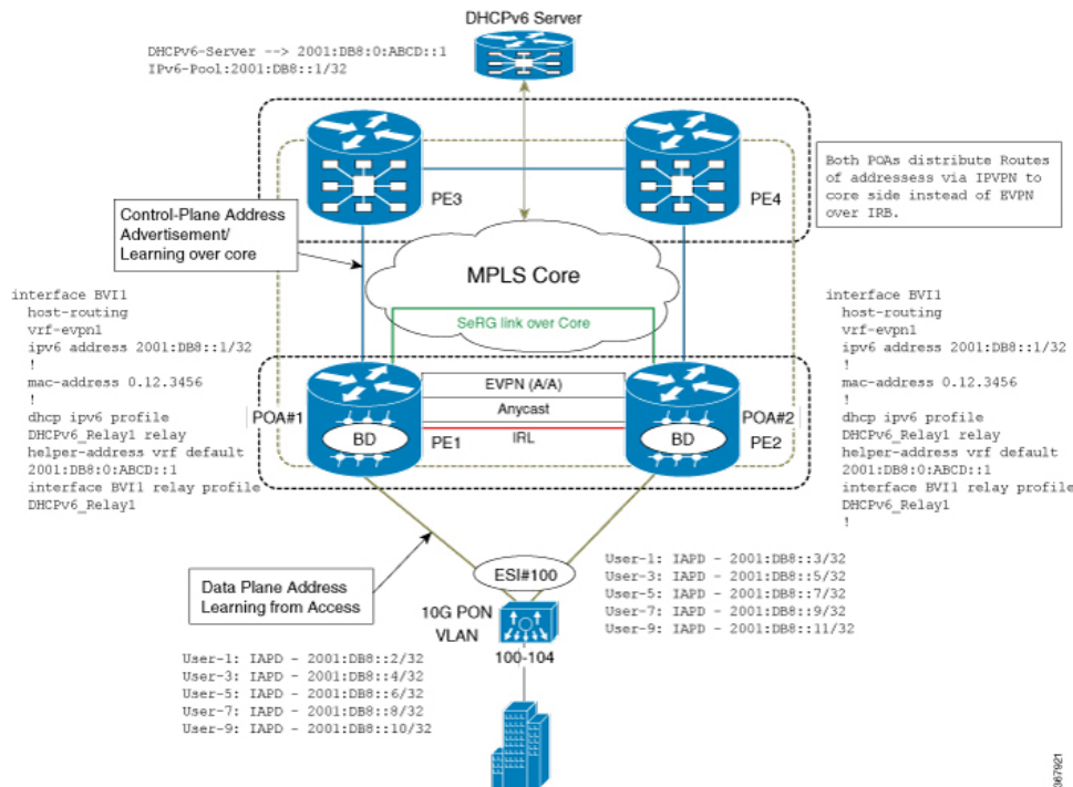
Figure 70: DHCPv6 relay Handling for EVPN and DHCPv6 Server in Default VRF
