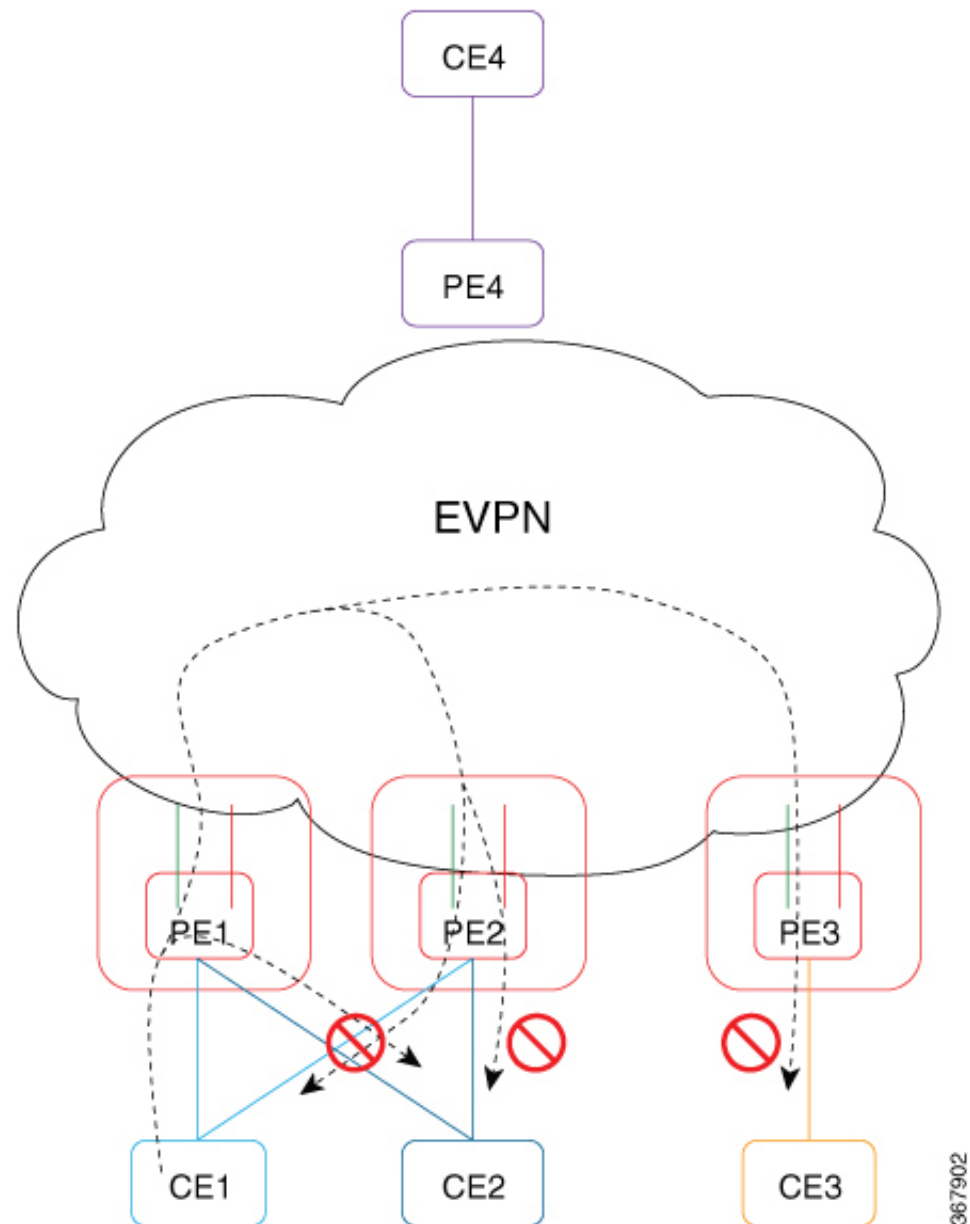
Figure 66: EVPN E-Tree
