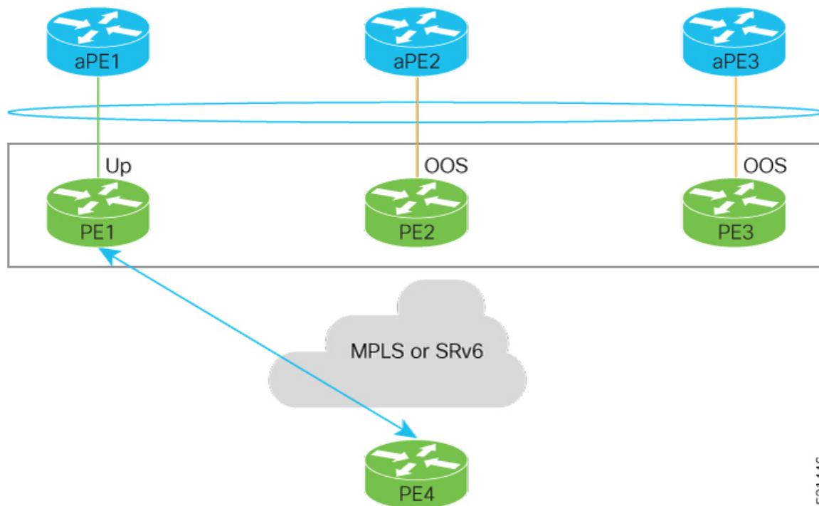
Figure 59: EVPN Access-Driven DF Election
