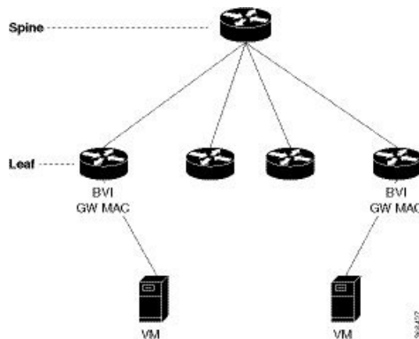
Figure 61: EVPN Single-Homing Access Gateway
