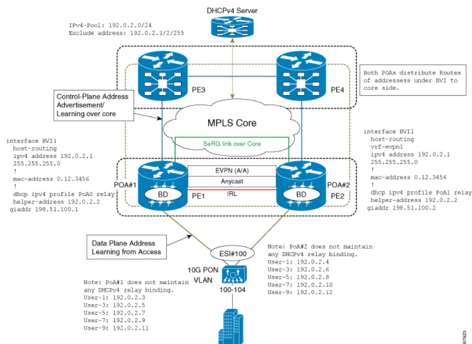
Figure 68: DHCPv4 Relay Handling for EVPN and DHCPv4 Server in Default VRF
