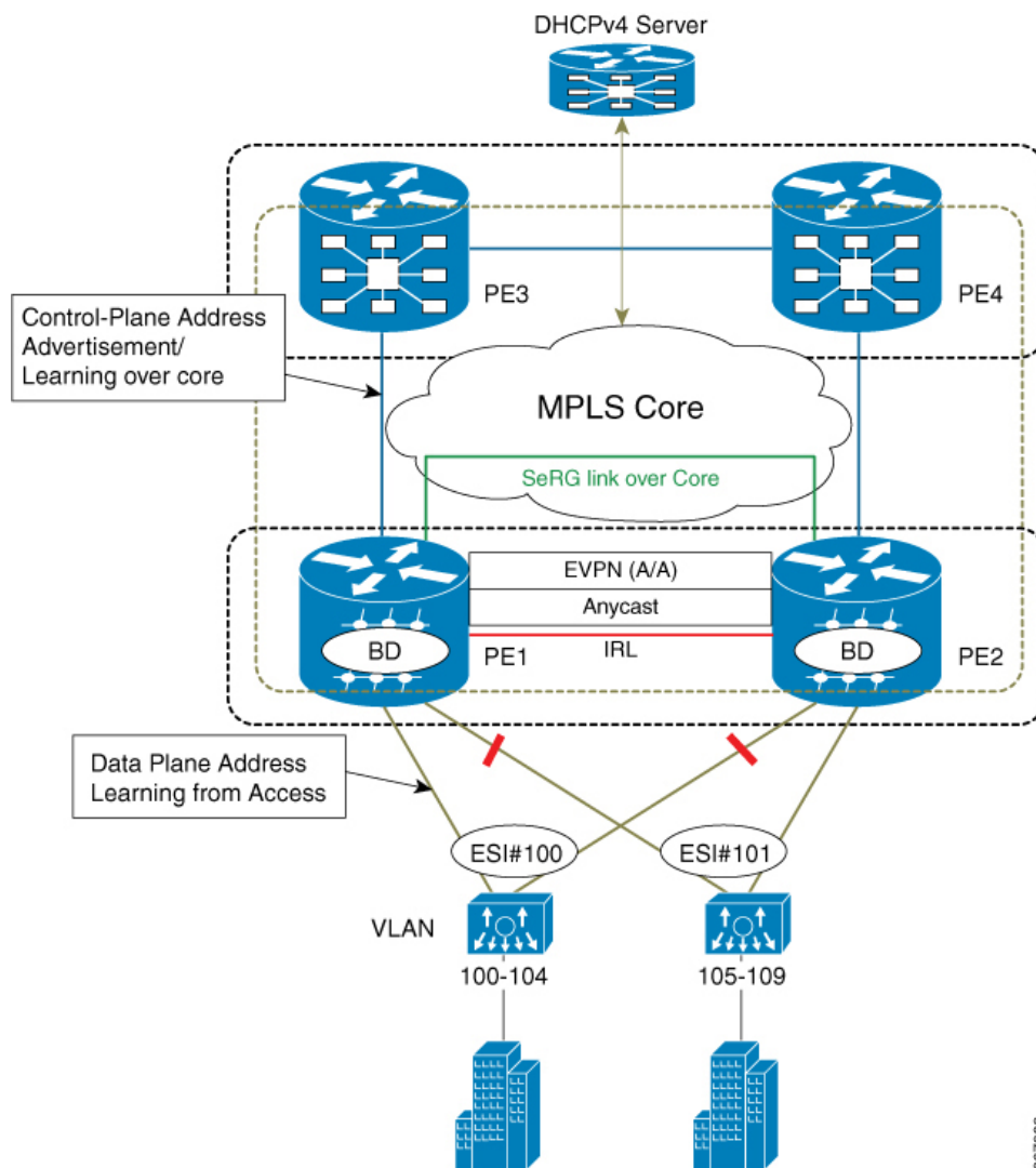
Figure 67: PON behavior in handling DHCPv4 Server for EVPN All-Active Multihoming
