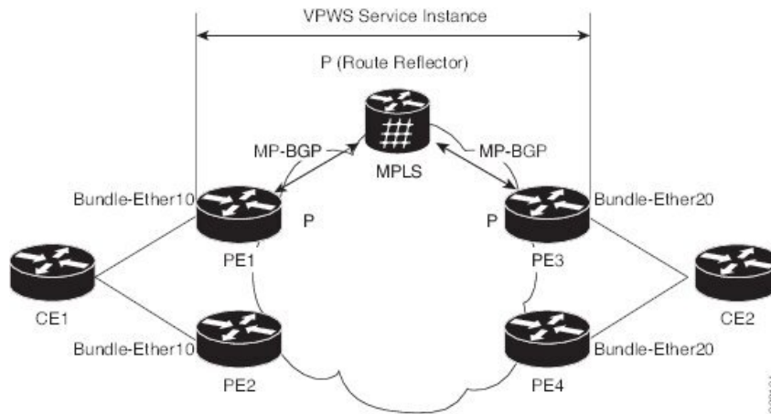
Figure 72: EVPN VPWS Multi-Homed
