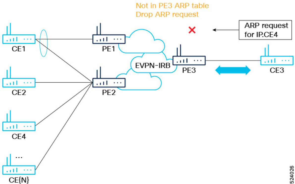
Figure 65: EVPN-IRB Network with ARP and ND Proxy Full Suppression
