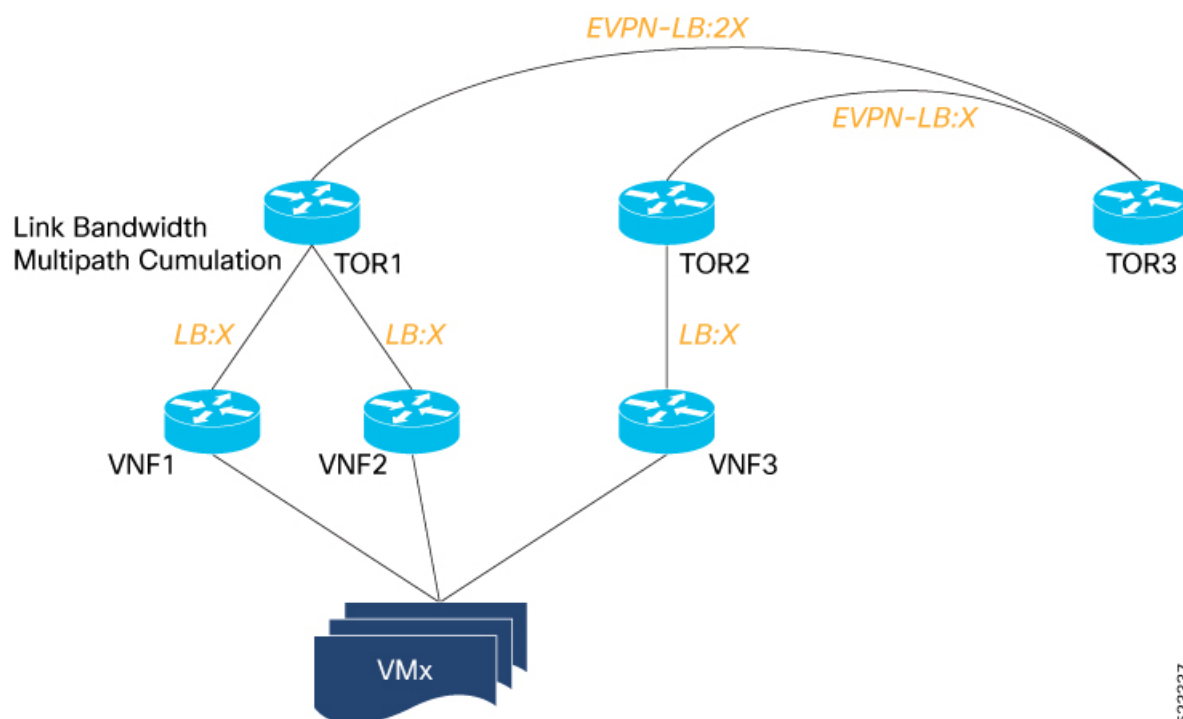
Figure 57: EVPN Link Bandwidth
