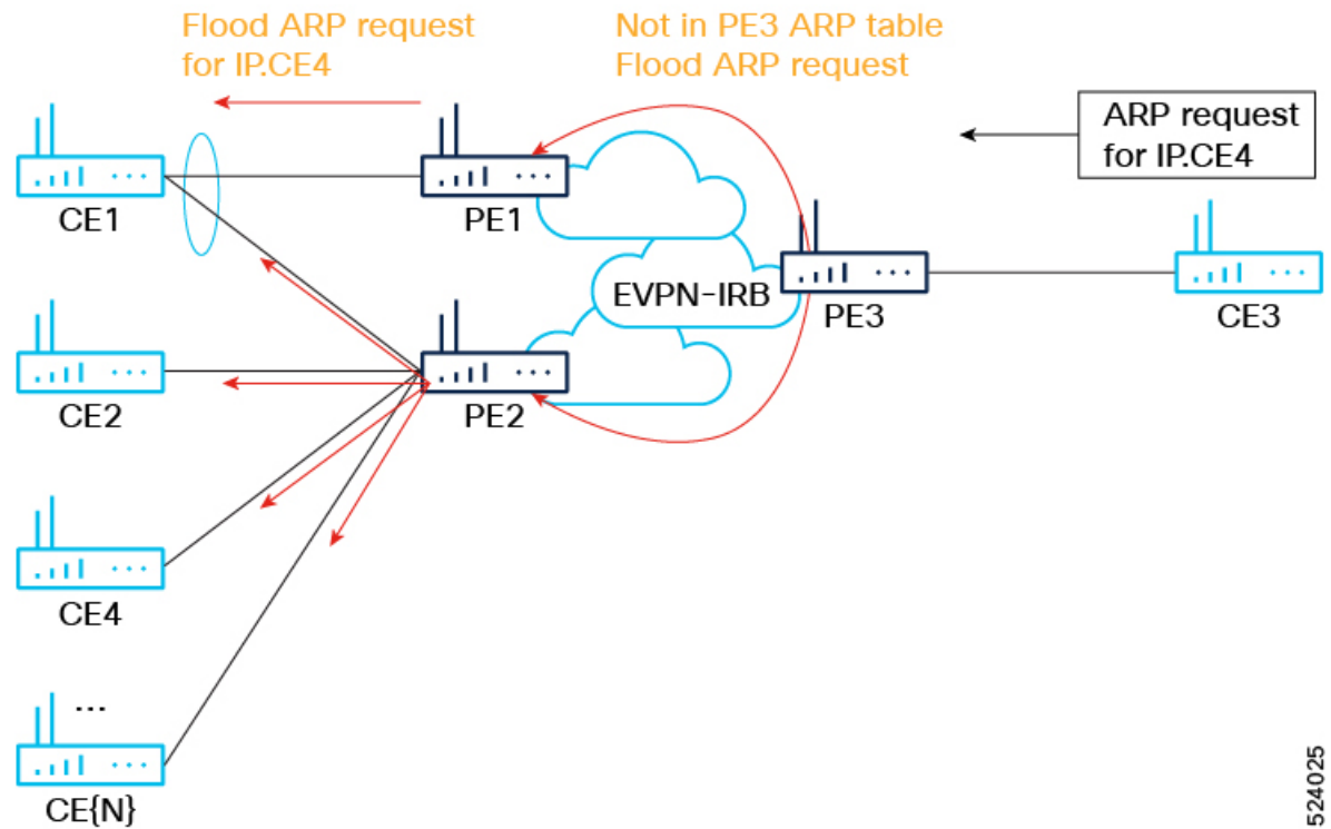
Figure 64: EVPN-IRB Network without ARP and ND Proxy Full Suppression or with ARP Proxy Partial Suppression
