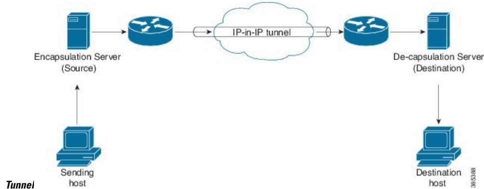
Figure 18: Basic Encapsulation and Decapsulation with an IP-in-IP
