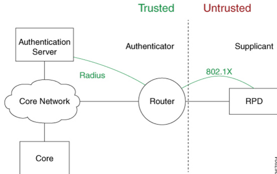
Figure 2: Topology for IEEE 802.1X Port-Based Authentication
