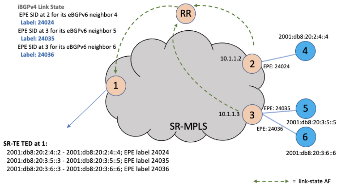
Figure 16: BGP-LS
