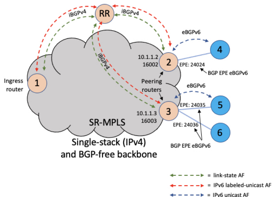
Figure 15: Network Setup
