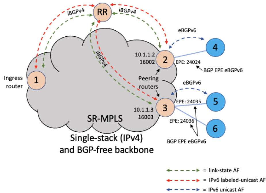
Figure 5: Network Setup
