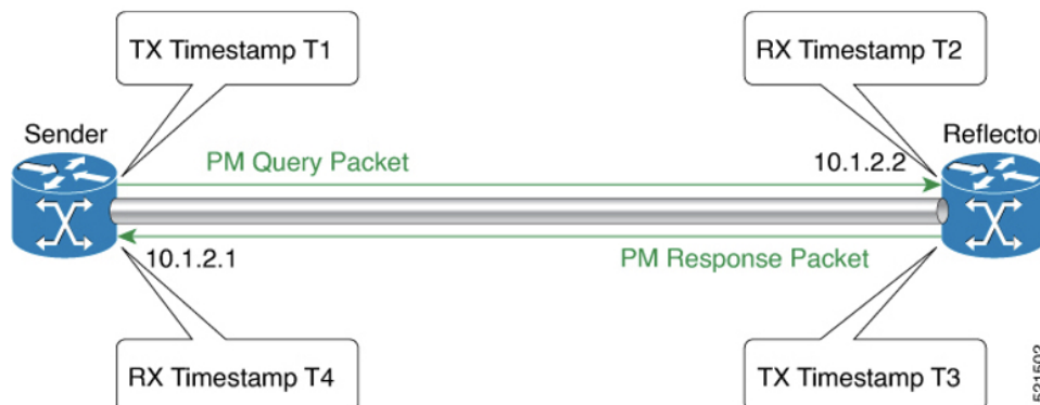
Figure 34: Two-Way
