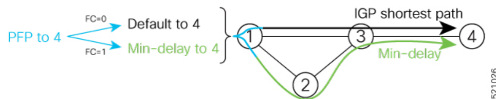
Figure 14: PFP Example
