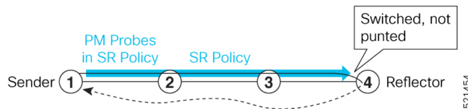
Figure 35: Loopback
