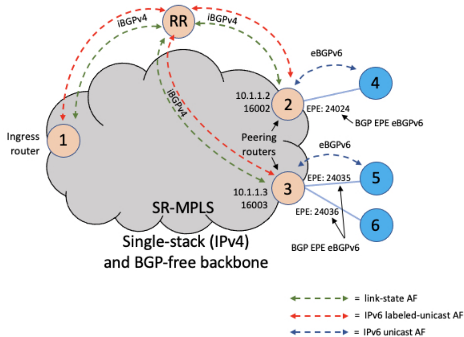
Figure 5: Network Setup
