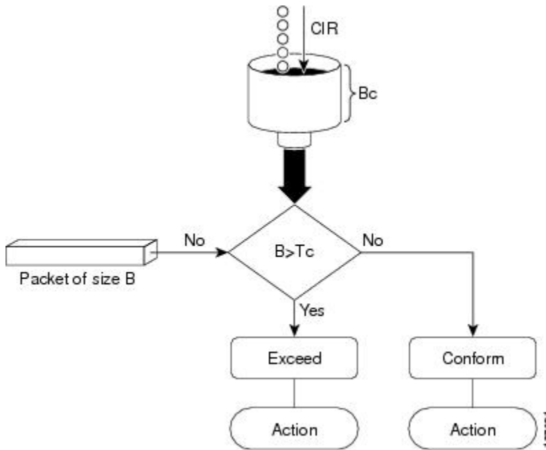
Figure 3: Workflow of Single-Rate Two-Color Policer
