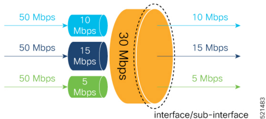
Figure 1: Parent Conform Aware-Ingress Policing
