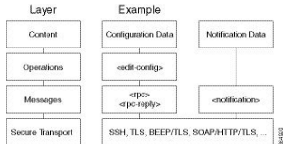
Figure 2: NETCONF Layers
