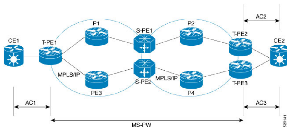
Figure 17: Multisegment Pseudowire Redundancy
