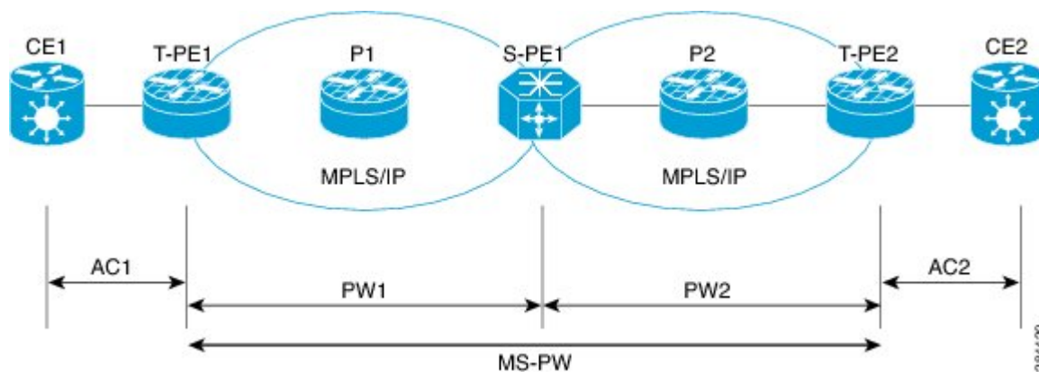
Figure 16: Multisegment Pseudowire
