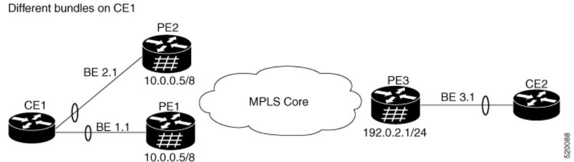
Figure 58: EVPN: Single-Active Multihoming for Anycast Gateway IRB
