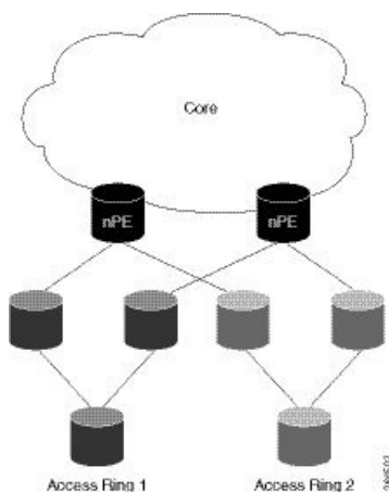
Figure 35: MSTAG Uplink Tracking
