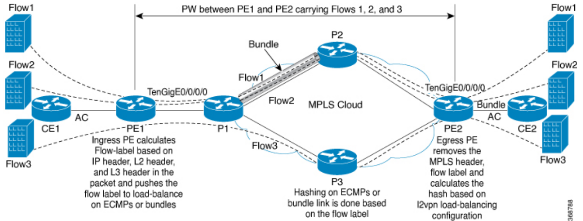
Figure 63: FAT PW with Two Flows Distributing over ECMPs and Bundle
