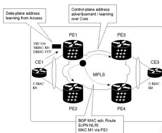
Figure 39: EVPN Operation
