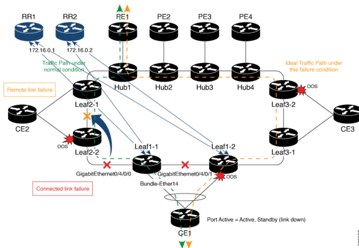
Figure 46: EVPN Convergence Using Core Isolation Protection
