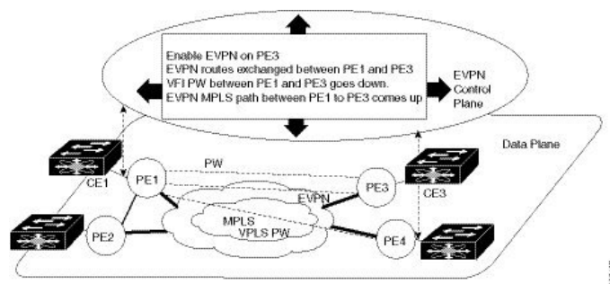
Figure 33: EVPN MPLS Seamless Integration with VPLS
