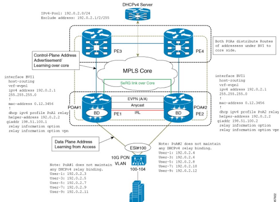
Figure 48: DHCPv4 Relay Handling for EVPN and DHCPv4 Server in Different VRF
