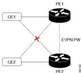
Figure 15: Local Switching
