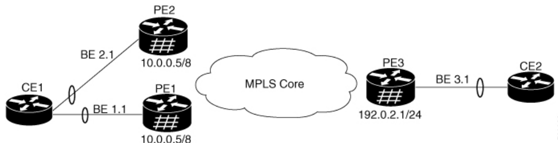
Figure 44: EVPN: Single-Active Multihoming for Anycast Gateway IRB
