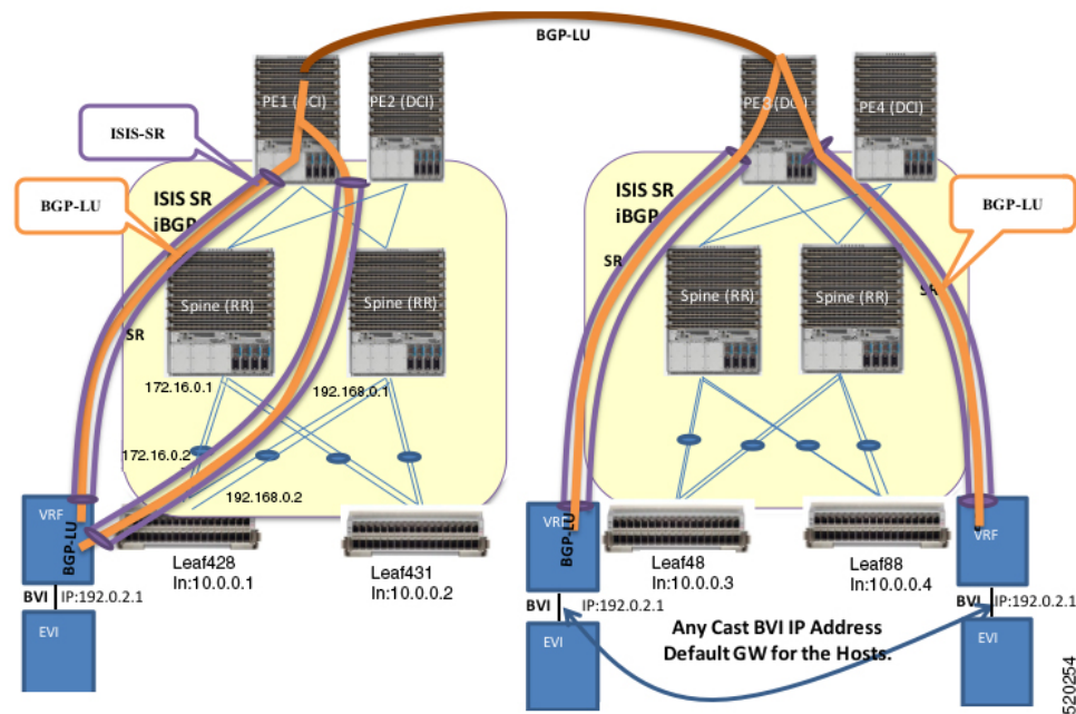
Figure 38: EVPN Bridging and VPWS Services over BGP-LU Underlay
