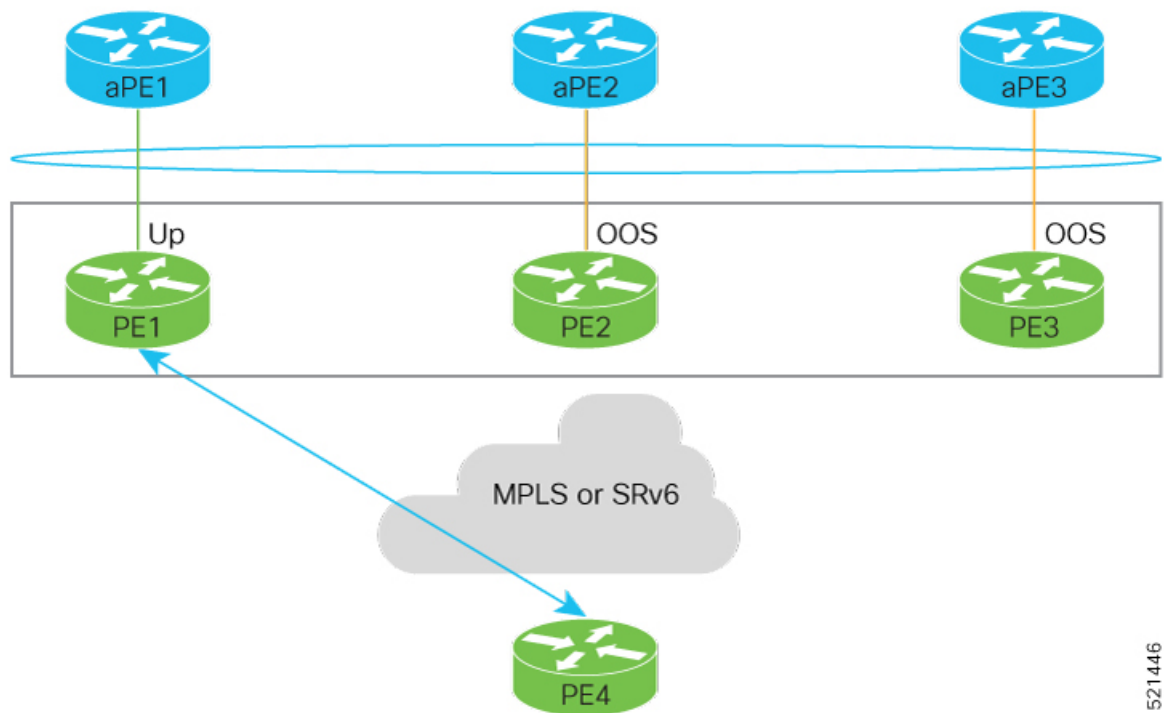
Figure 40: EVPN Access-Driven DF Election
