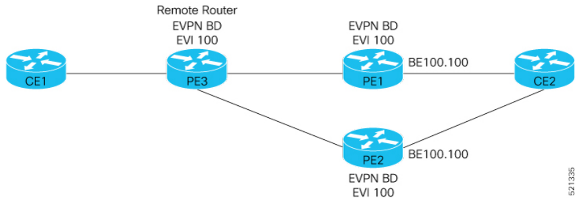
Figure 39: Layer 2 Fast Reroute
