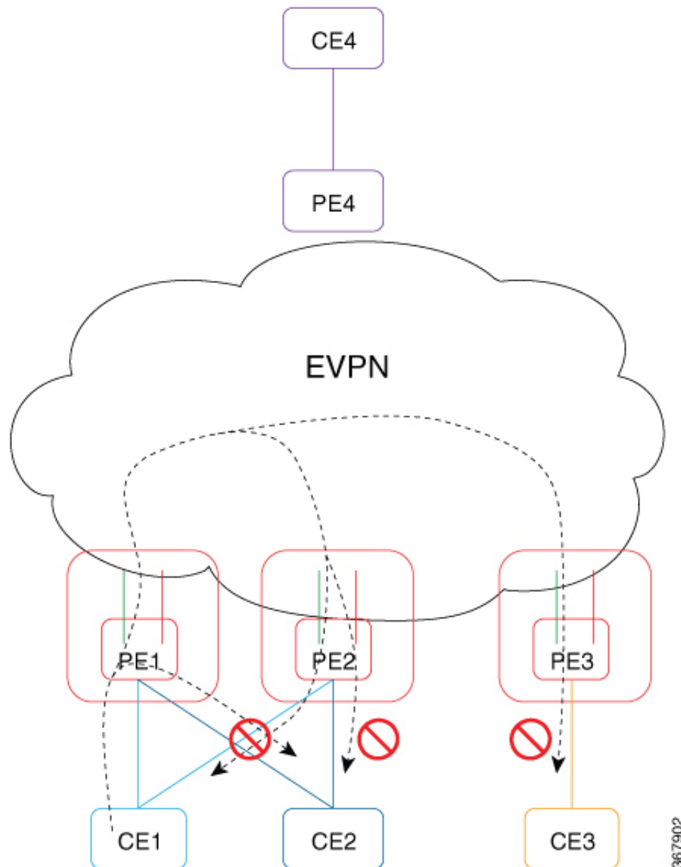
Figure 45: EVPN E-Tree
