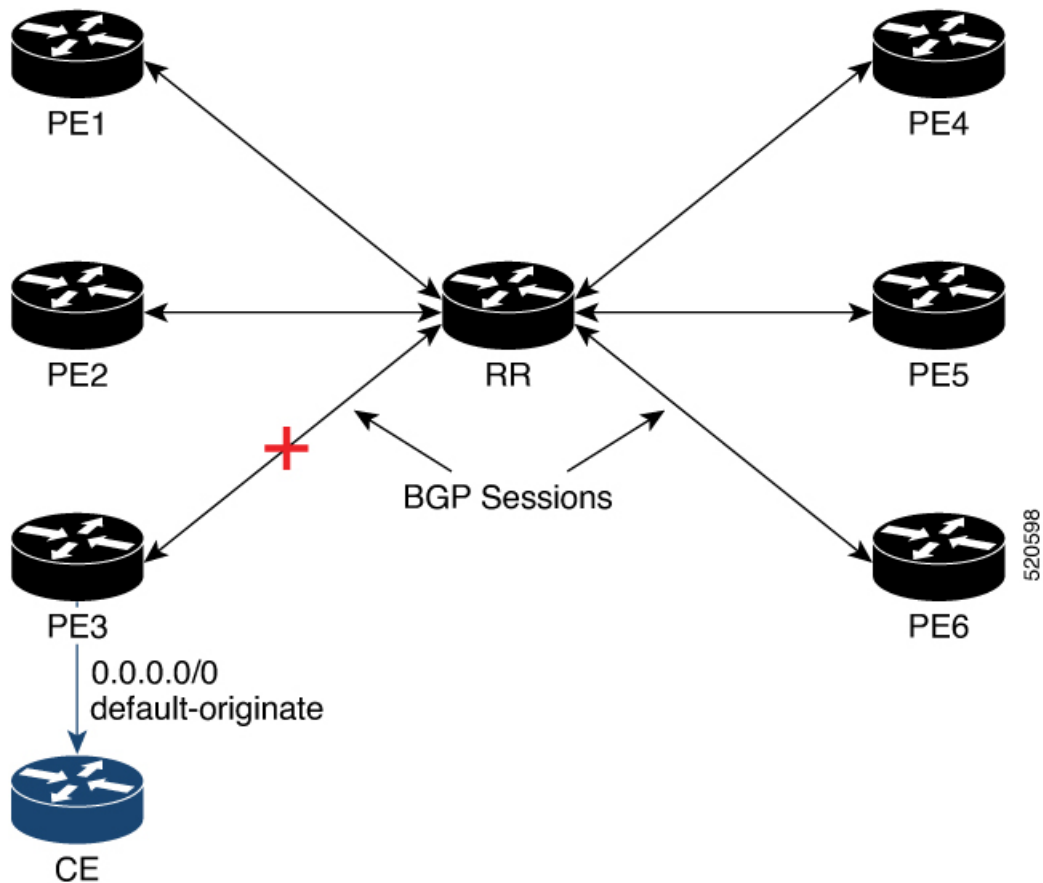
Figure 36: Advertisement of default-originate
