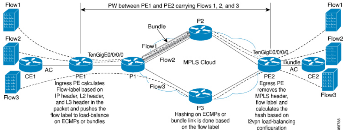
Figure 7: FAT PW with Two Flows Distributing over ECMPs and Bundle
