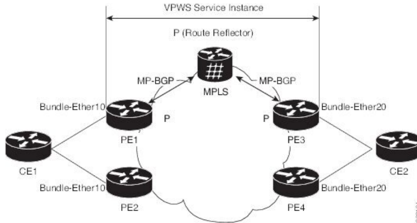
Figure 50: EVPN VPWS Multi-Homed
