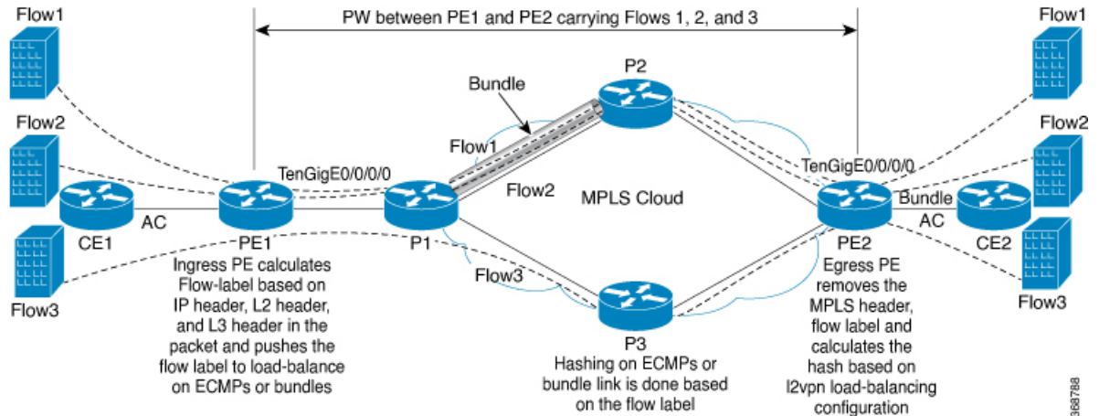
Figure 51: FAT PW with Two Flows Distributing over ECMPs and Bundle
