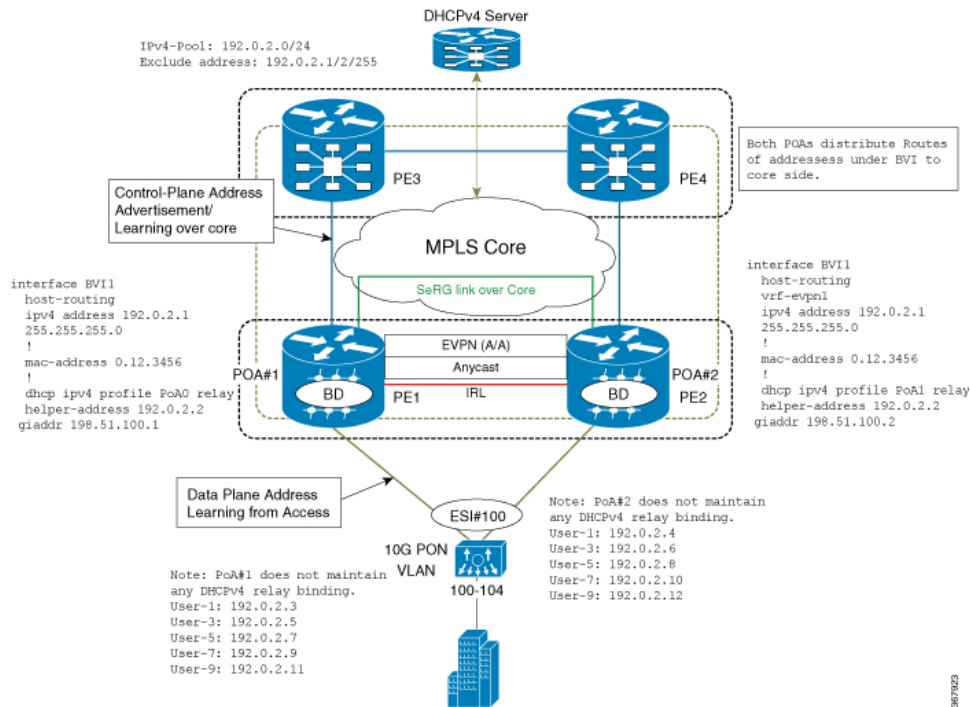
Figure 47: DHCPv4 Relay Handling for EVPN and DHCPv4 Server in Default VRF
