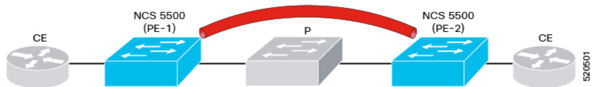
Figure 1: L2CP Tunneling
