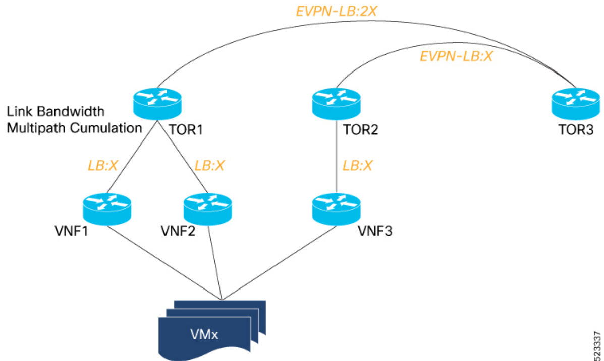
Figure 17: EVPN Link Bandwidth
