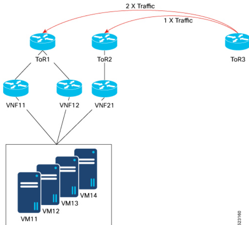
Figure 16: Proportional Multipath
