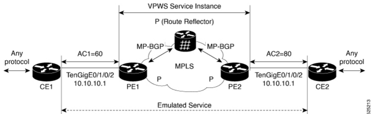
Figure 3: VPWS Traffic flow
