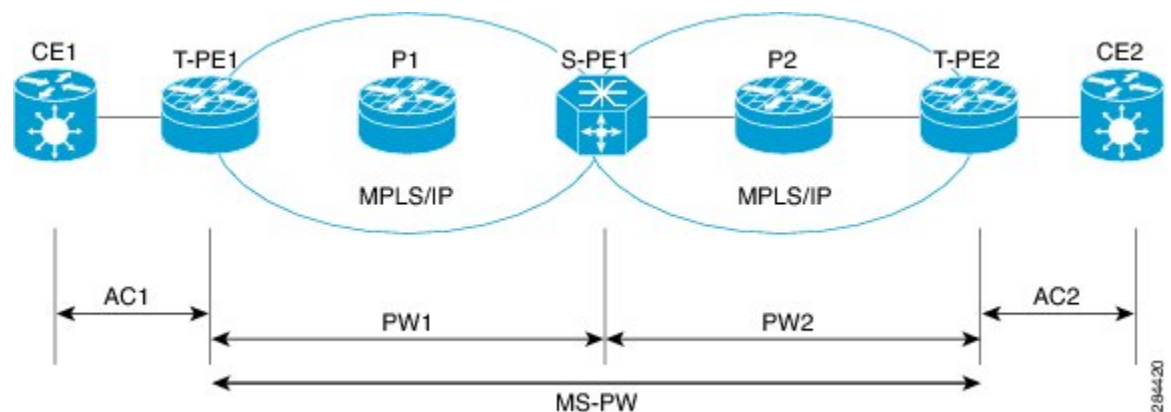
Figure 9: Multisegment Pseudowire
