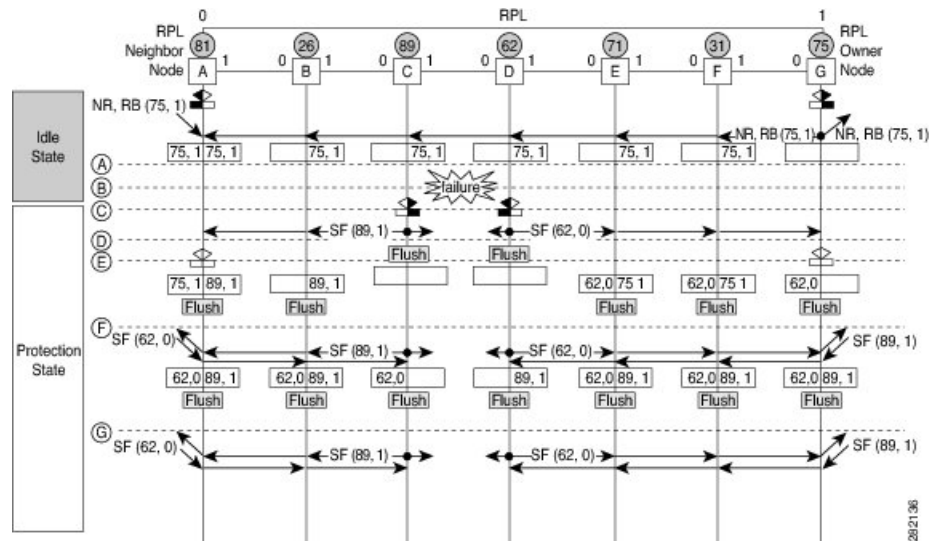
Figure 13: G.8032 Single Link Failure
