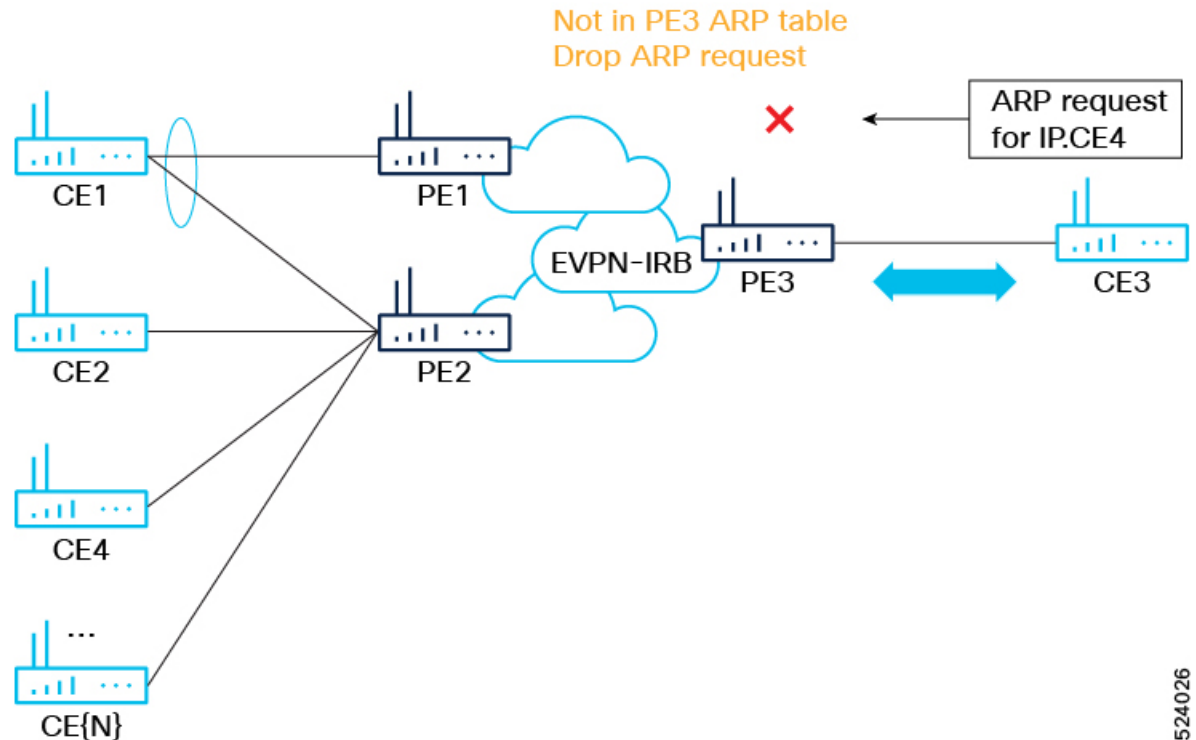
Figure 64: EVPN-IRB Network with ARP and ND Proxy Full Suppression
