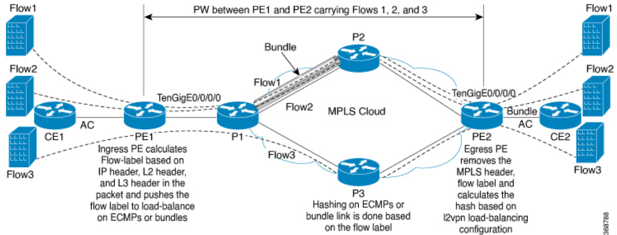
Figure 71: FAT PW with Two Flows Distributing over ECMPs and Bundle
