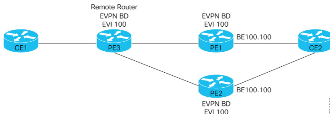
Figure 57: Layer 2 FRR multi-homing topology
