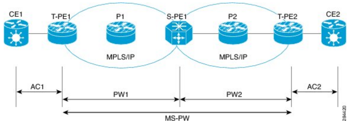
Figure 16: Multisegment Pseudowire
