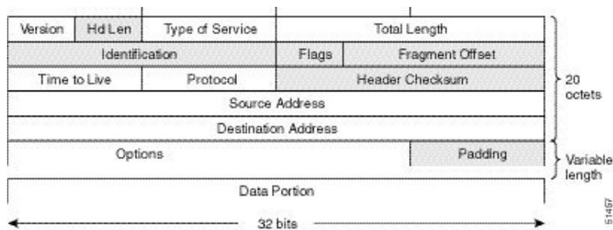
Figure 4: IPv4 Packet Header Format
