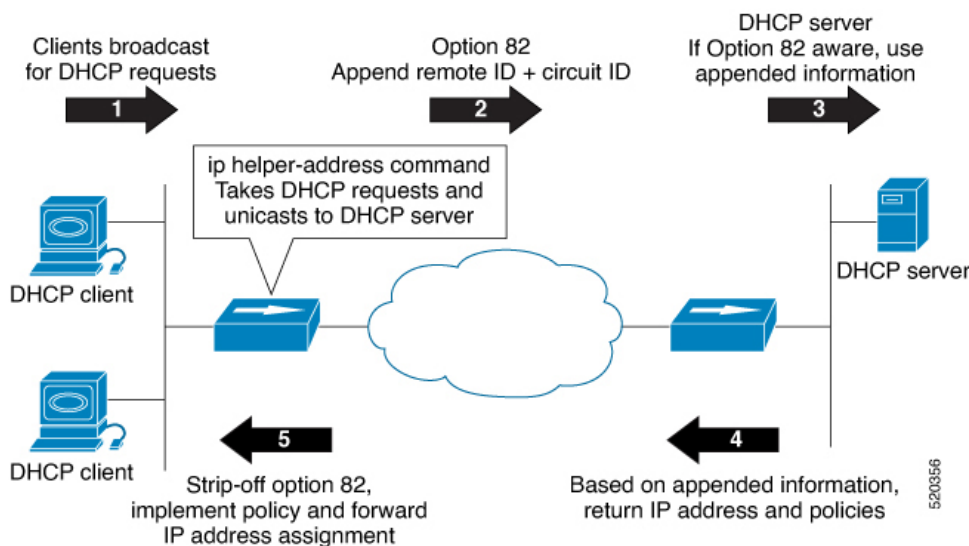
Figure 1: Forwarding Packets Using DHCP Relay Option-82
