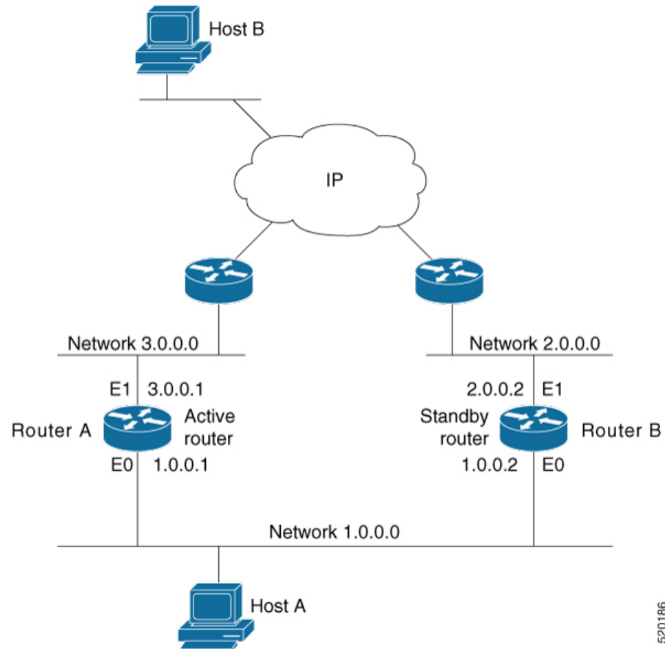
Figure 12: Routers Configured as an HSRP Group
