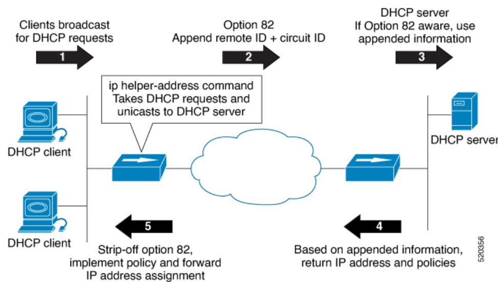
Figure 2: Forwarding Packets Using DHCP Relay Option-82
