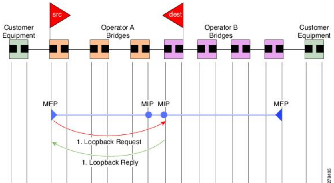
Figure 6: Loopback Messages
