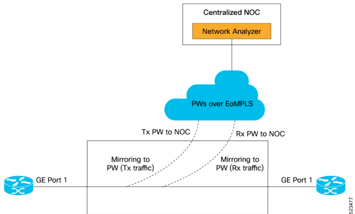
Figure 3: Mirroring Topology
