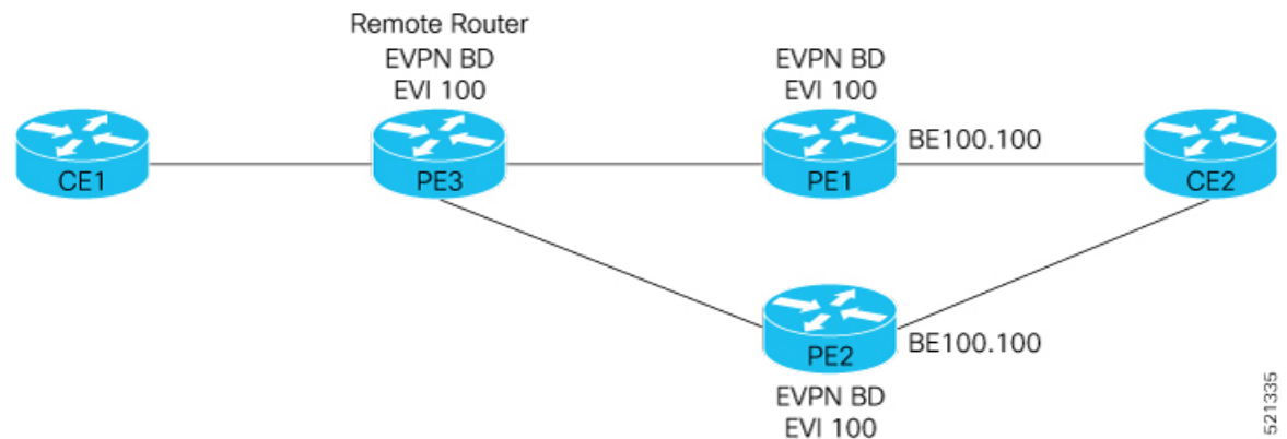
Figure 14: Layer 2 Fast Reroute
