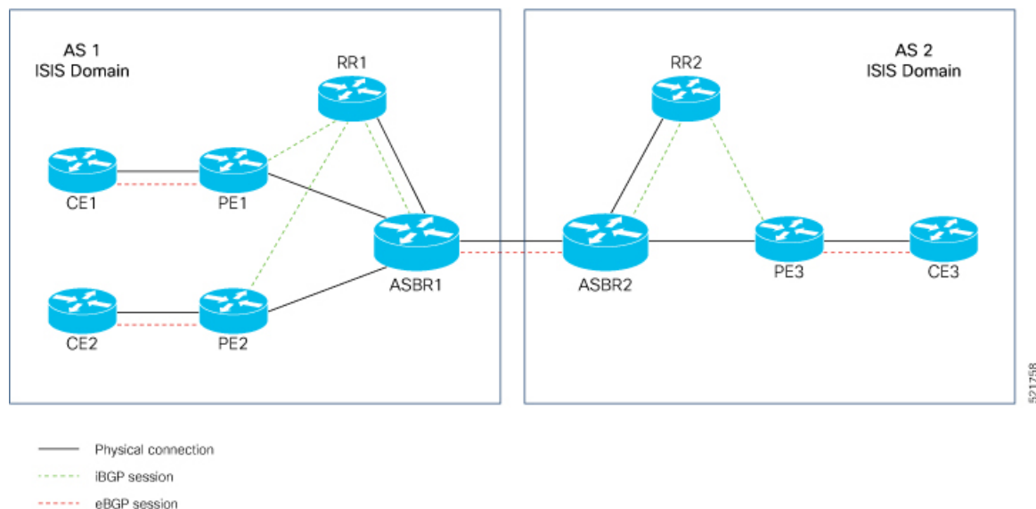
Figure 16: Inter-AS EVPN Option B
