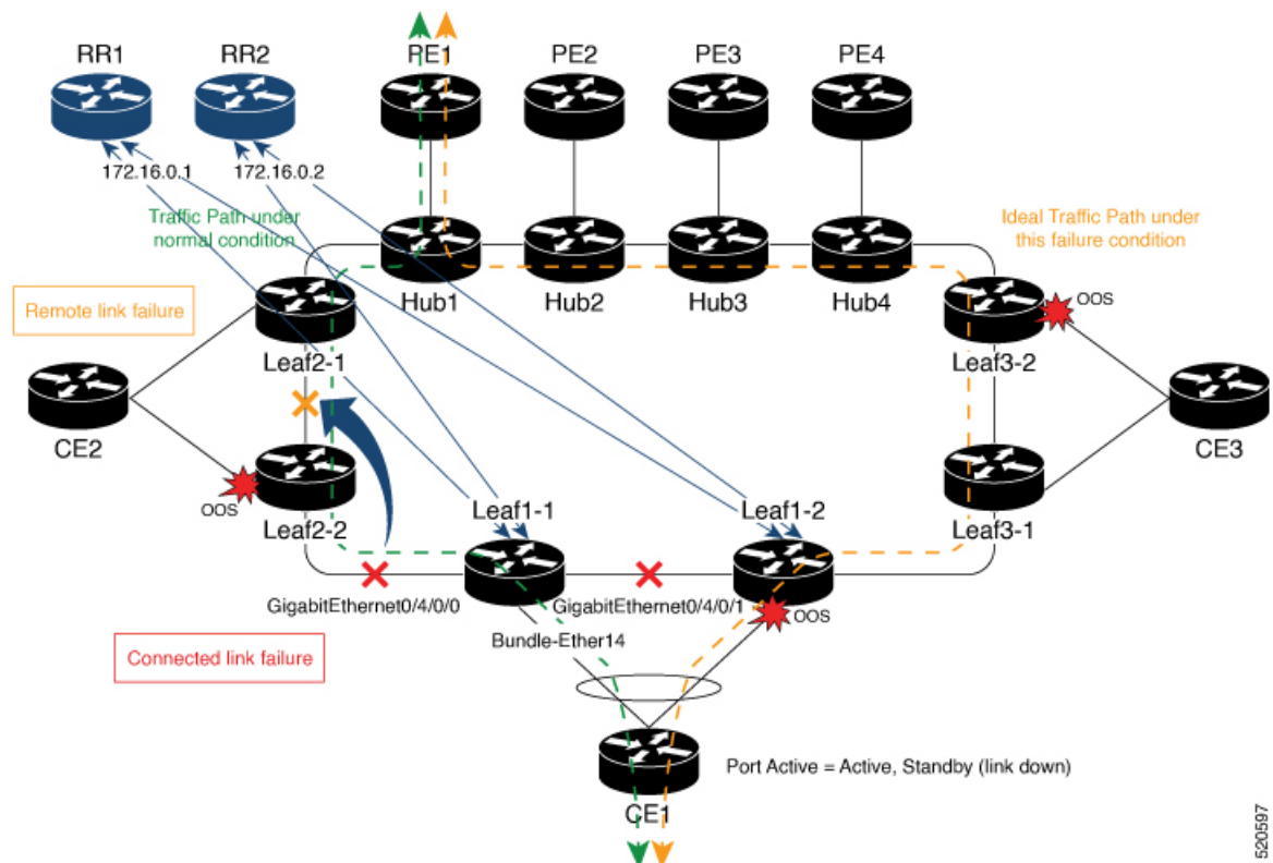
Figure 11: EVPN Convergence Using Core Isolation Protection
