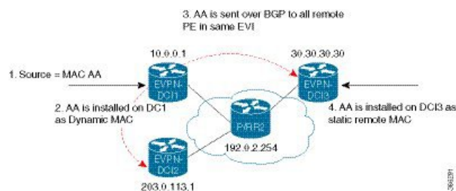
Figure 5: EVPN Software MAC Learning
