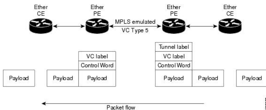
Figure 11: Ethernet Port Mode Packet Flow
