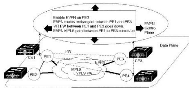
Figure 37: EVPN MPLS Seamless Integration with VPLS
