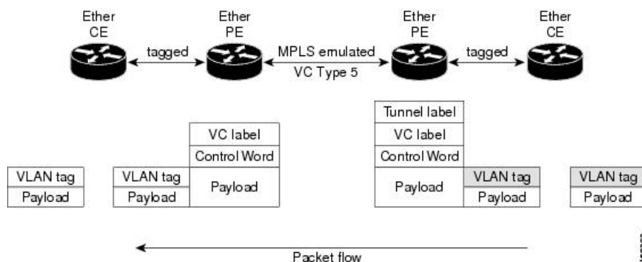
Figure 12: VLAN Mode Packet Flow
