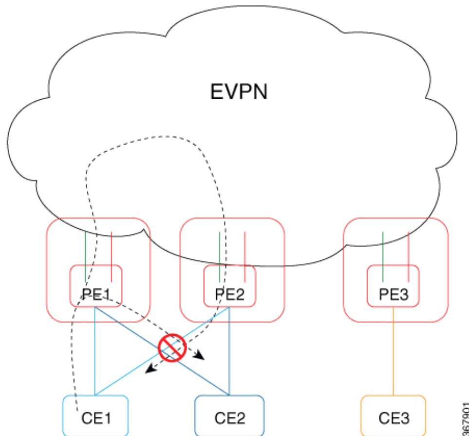
Figure 10: Topology
