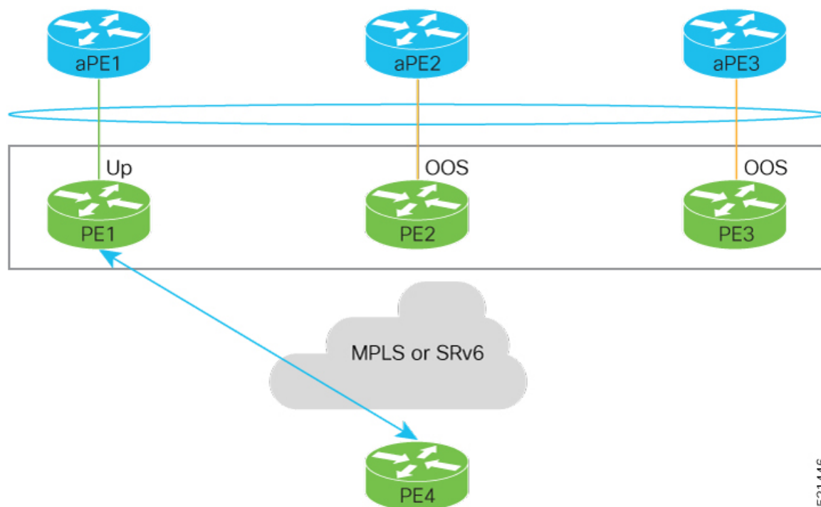
Figure 12: EVPN Access-Driven DF Election
