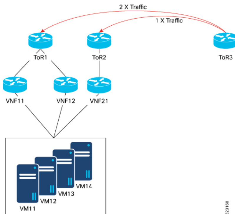
Figure 20: Proportional Multipath
