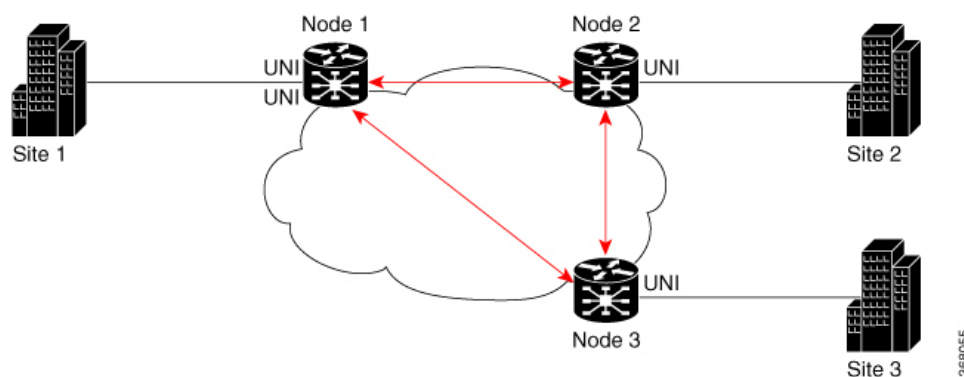
Figure 18: CFM on EVPN ELAN: Full Mesh Topology
