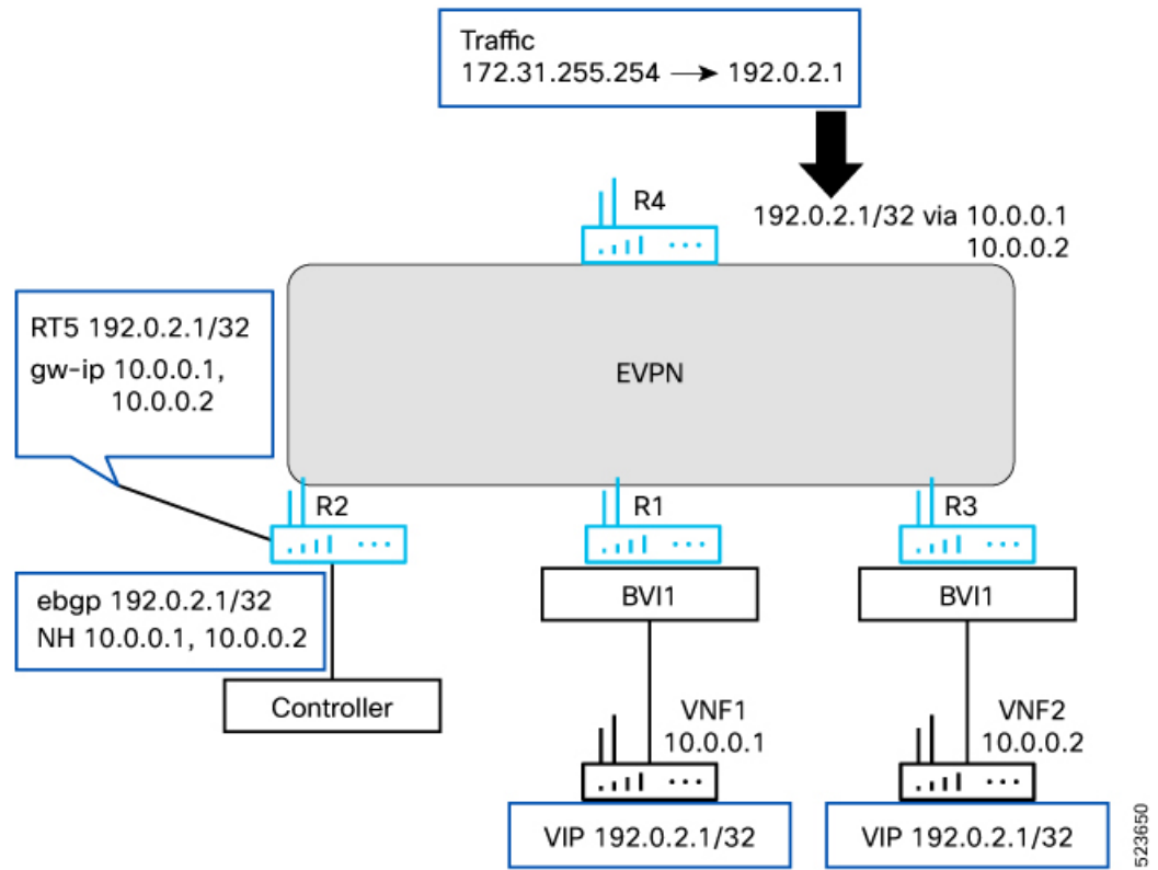
Figure 21: Host tracking using BFD
