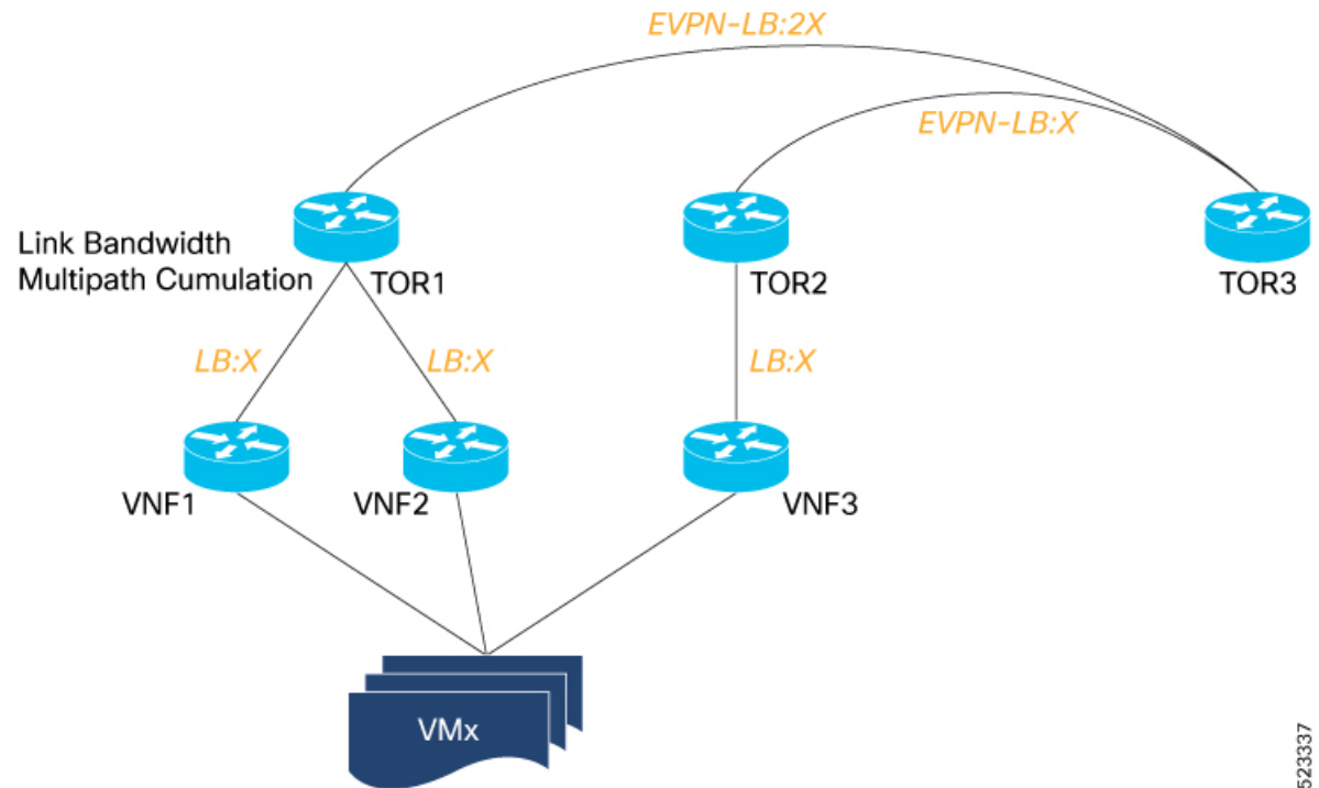
Figure 22: EVPN Link Bandwidth
