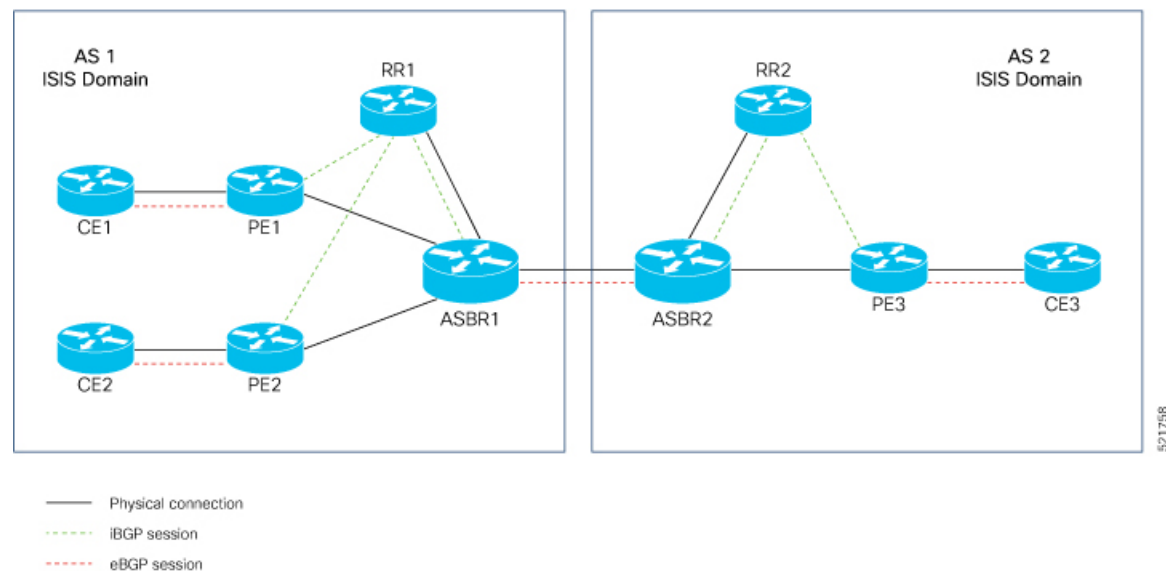
Figure 56: Inter-AS EVPN Option B
