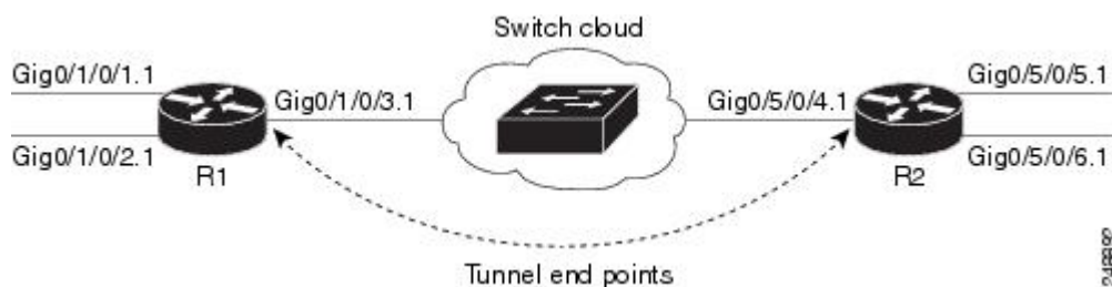
Figure 5: L2PT in forward mode
