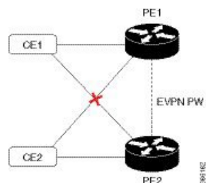
Figure 23: Local Switching
