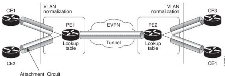
Figure 21: Flexible Cross-Connect Service
