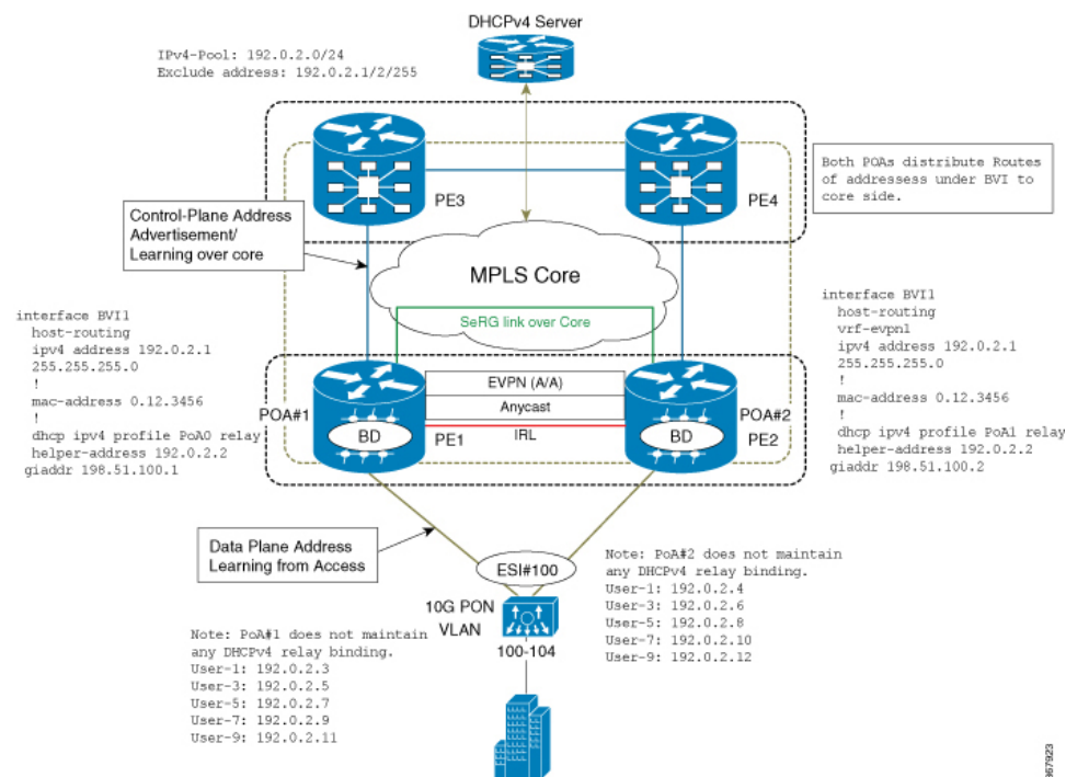
Figure 73: DHCPv4 Relay Handling for EVPN and DHCPv4 Server in Default VRF
