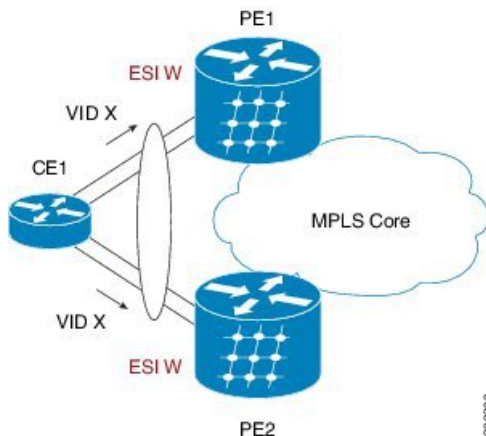
Figure 46: Dual Home Device —All-Active Load Balancing Mode
