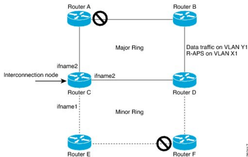
Figure 31: Open Ring Scenario - interconnection node
