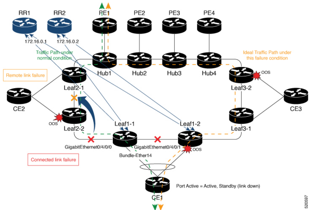
Figure 50: EVPN Convergence Using Core Isolation Protection
