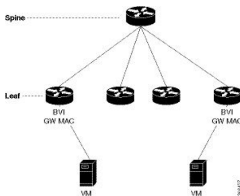
Figure 65: EVPN Single-Homing Access Gateway
