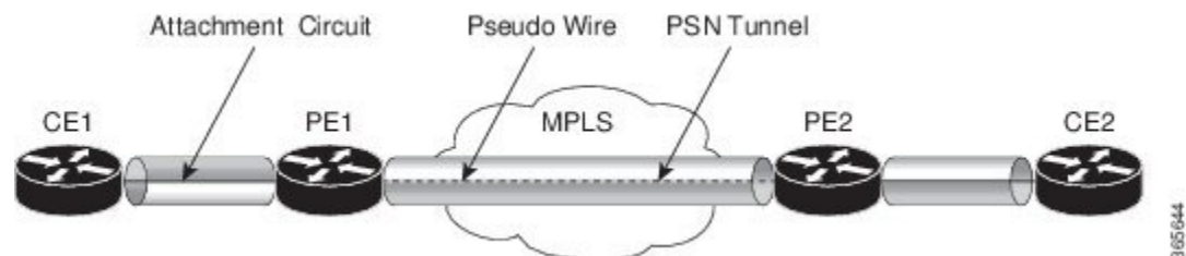
Figure 20: Static Cross-Connect Circuits in a Layer 2 VPN
