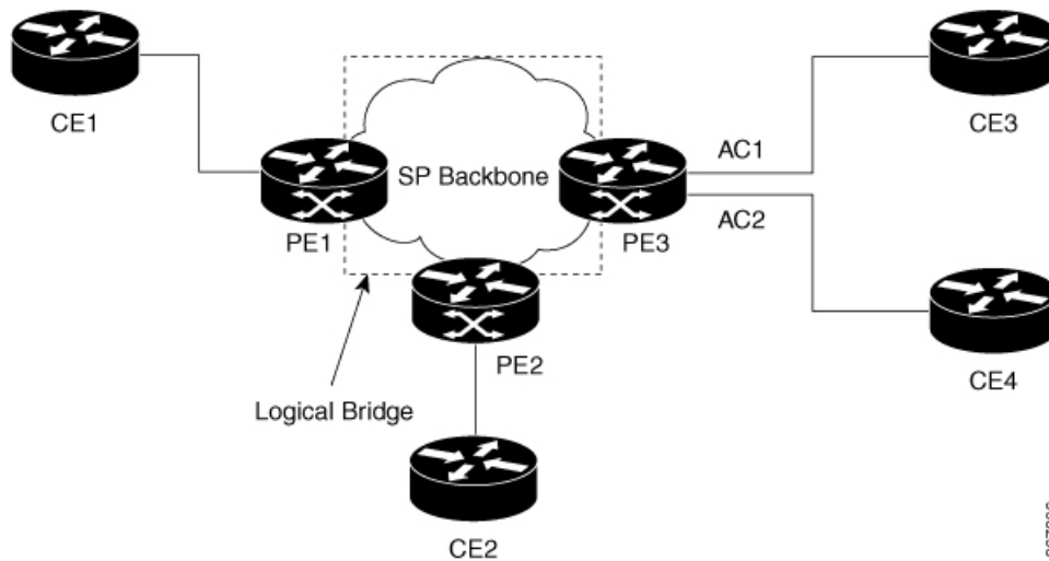
Figure 27: Split Horizon Group 2
