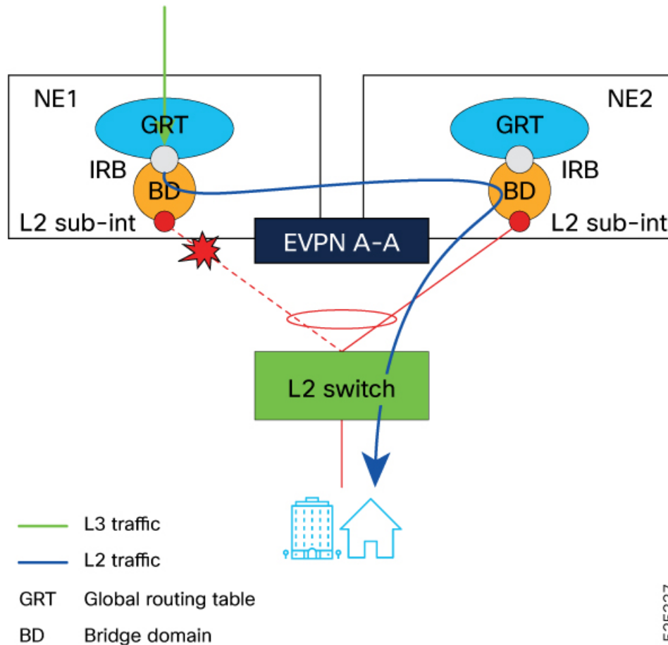
Figure 76: Topology for EVPN active-active multi-homing
