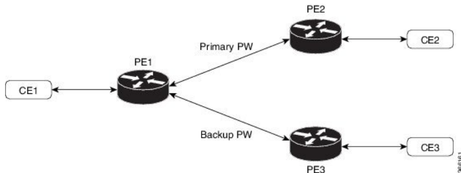
Figure 34: Access Pseudowire Redundancy
