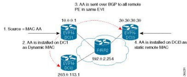
Figure 44: EVPN Software MAC Learning
