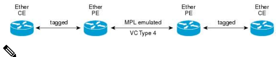
Figure 18: EoMPLS over QinQ Mode
