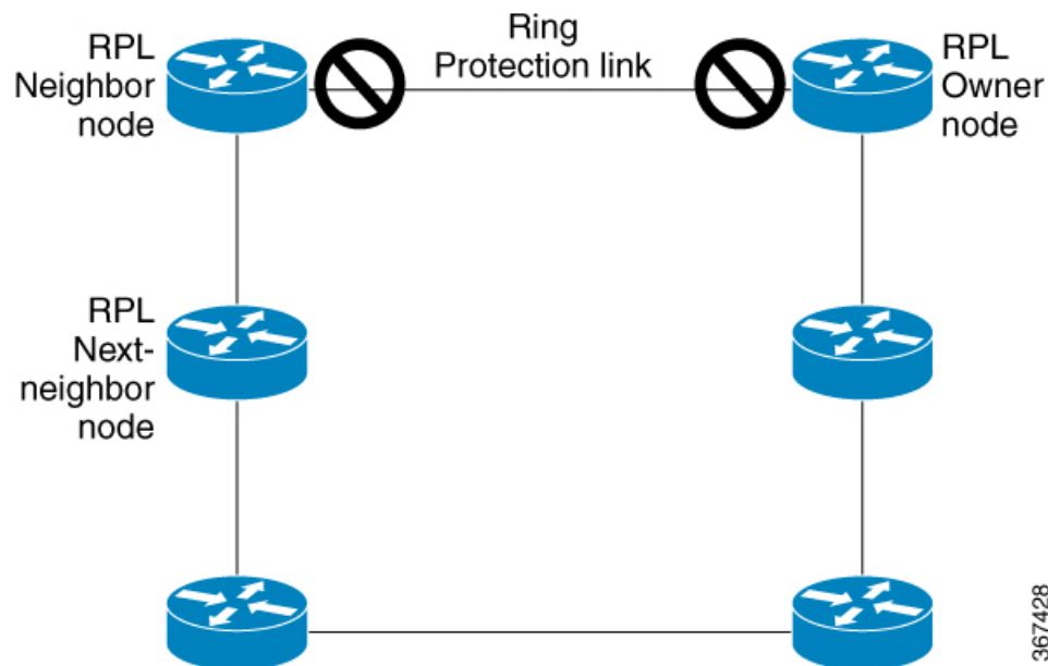
Figure 28: G.8032 Ethernet Ring
