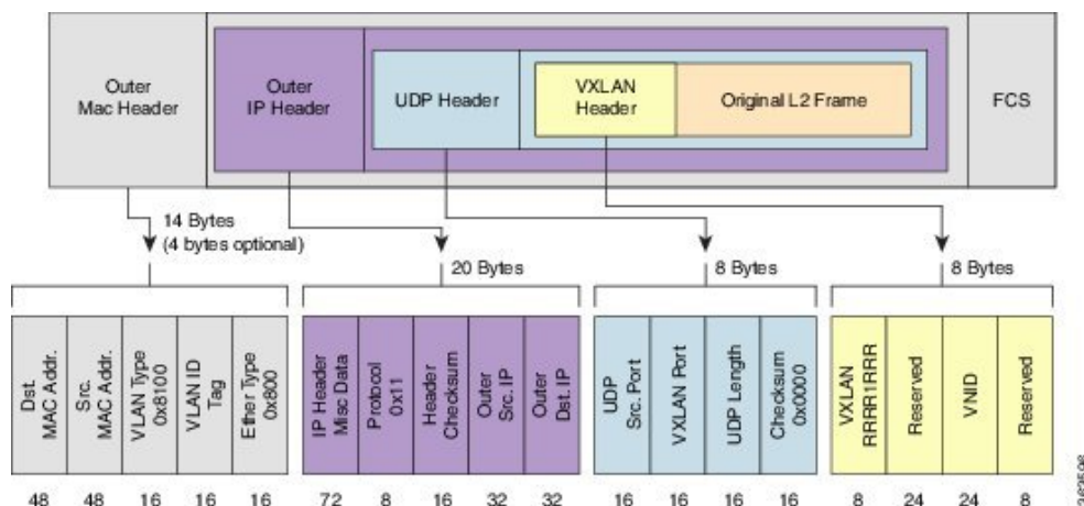
Figure 88: VXLAN Packet Format
