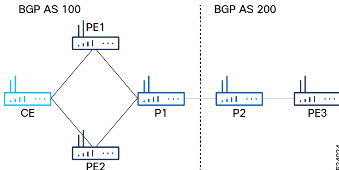
Figure 57: Inter-AS option C
