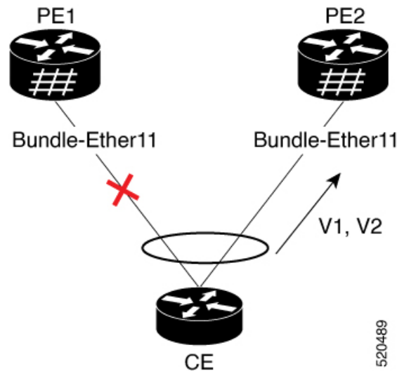
Figure 41: EVPN Port-Active Multihoming
