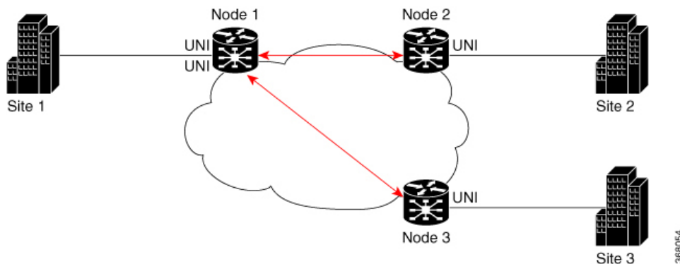
Figure 60: CFM on EVPN ELAN: Hub and Spoke Topology
