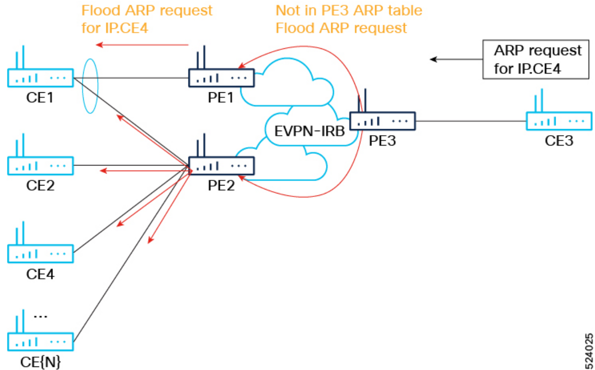
Figure 69: EVPN-IRB Network without ARP and ND Proxy Full Suppression or with ARP Proxy Partial Suppression
