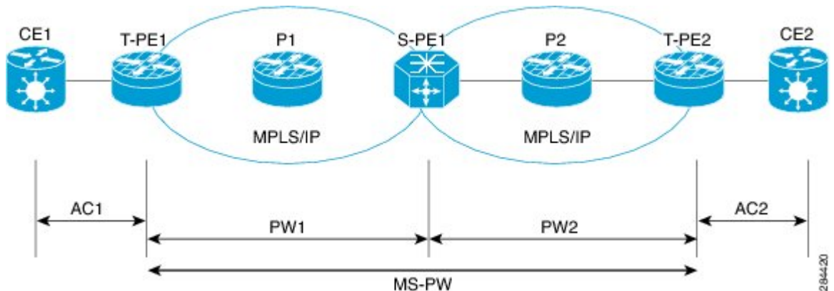
Figure 25: Multisegment Pseudowire
