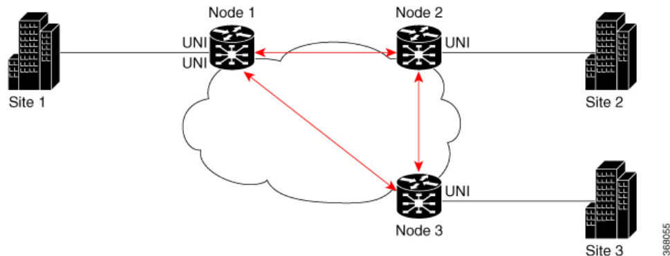
Figure 80: CFM on EVPN VPWS: Full Mesh Topology
