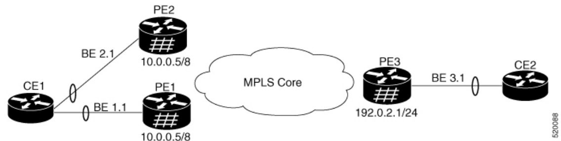
Figure 67: EVPN: Single-Active Multihoming for Anycast Gateway IRB
