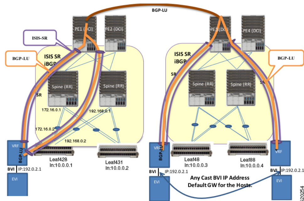
Figure 52: EVPN Bridging and VPWS Services over BGP-LU Underlay
