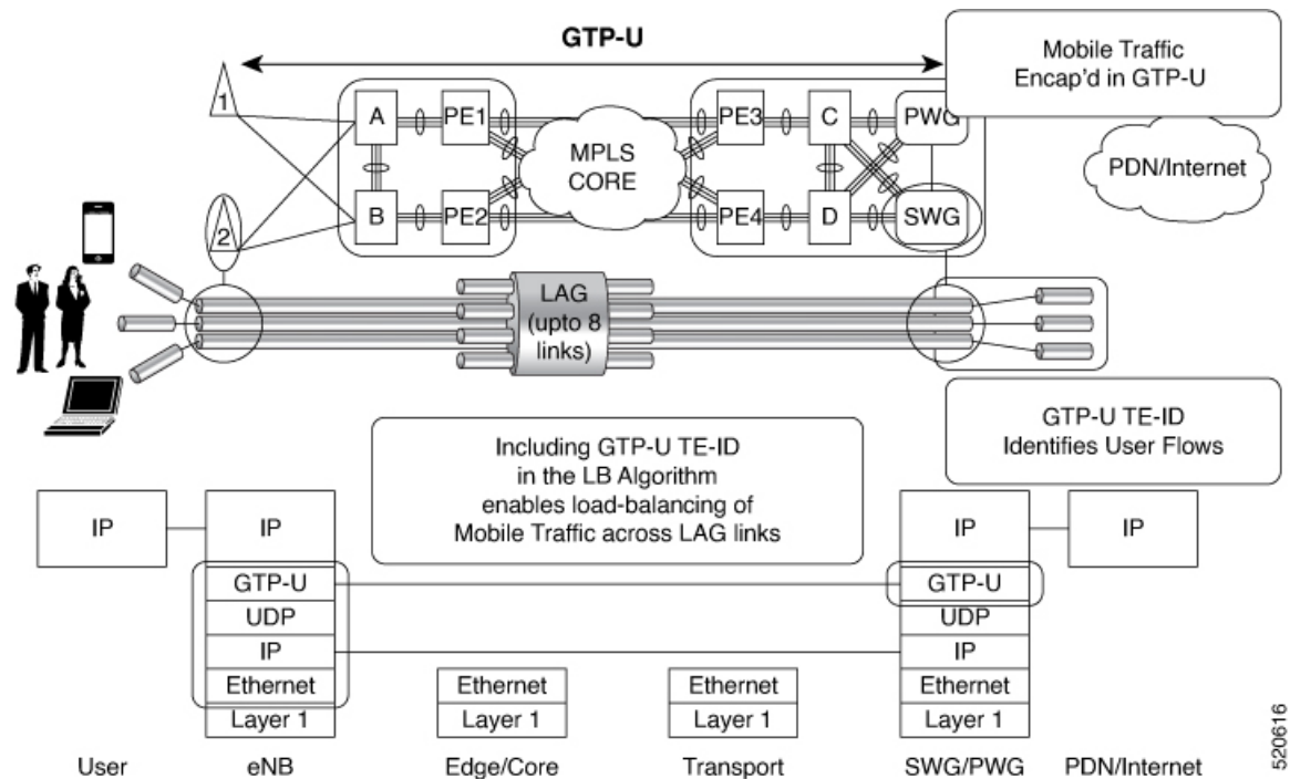
Figure 35: Mobile Transport GTP-U Load-Balancing
