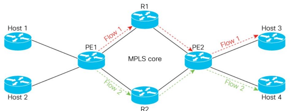
Figure 13: Fat label-based load balancing on L2VPN decapsulation node workflow
