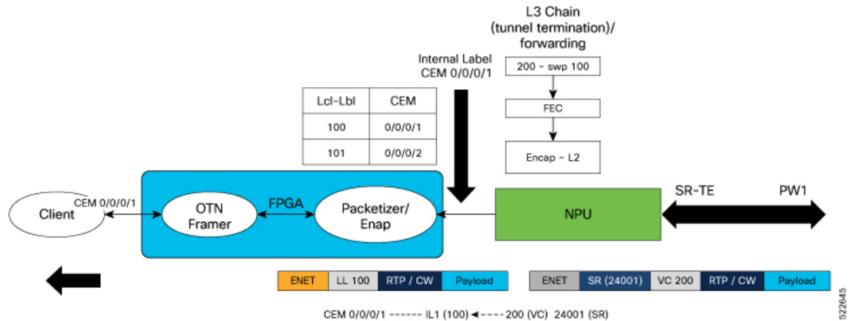
Figure 82: PLE Forwarding Flow – Disposition
