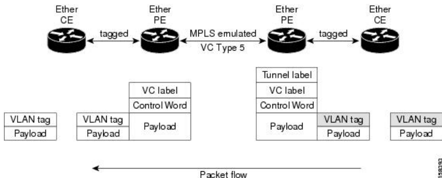
Figure 16: VLAN Mode Packet Flow
