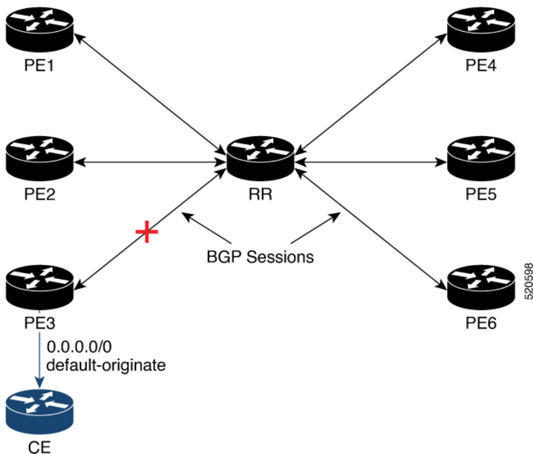
Figure 51: Advertisement of default-originate
