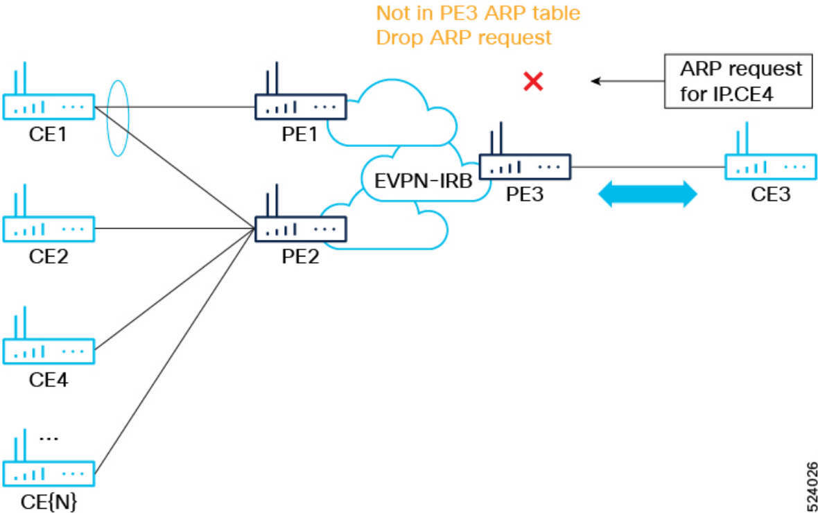
Figure 70: EVPN-IRB Network with ARP and ND Proxy Full Suppression
