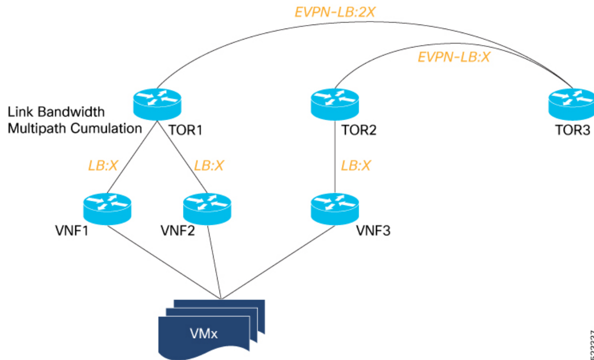
Figure 63: EVPN Link Bandwidth
