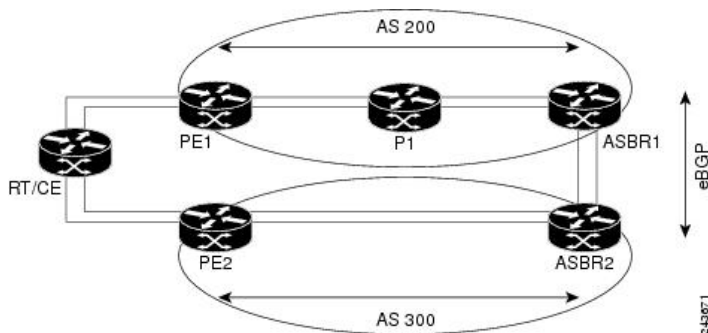
Figure 17: EoMPLS over Inter-AS: Basic Double AS Topology
