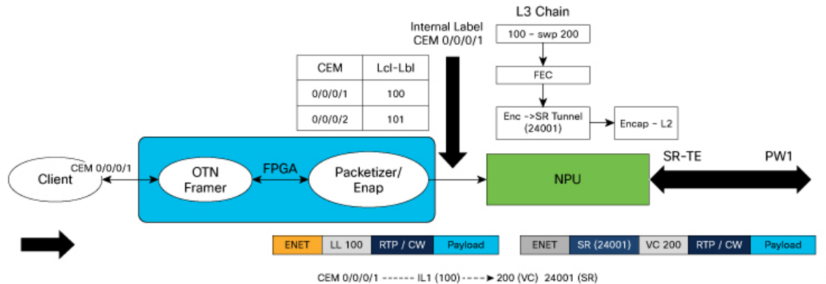
Figure 81: PLE Forwarding Flow – Imposition
