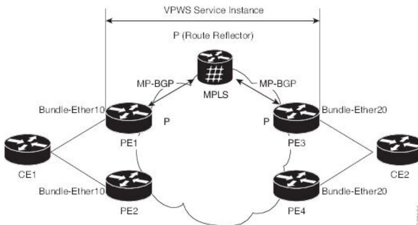
Figure 54: Layer 2 FRR multi-homing topology
