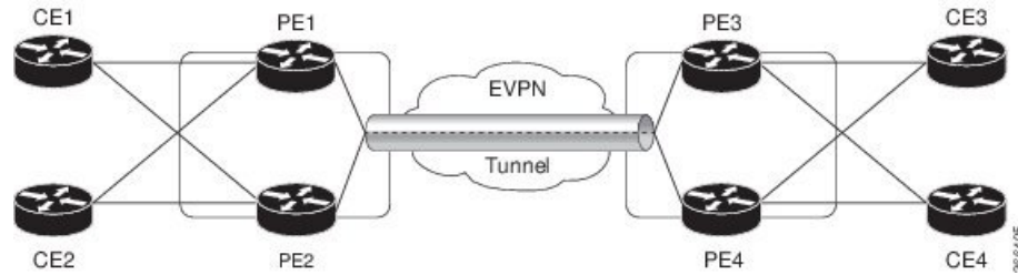
Figure 22: Flexible Cross-Connect Service Multi-Homed
