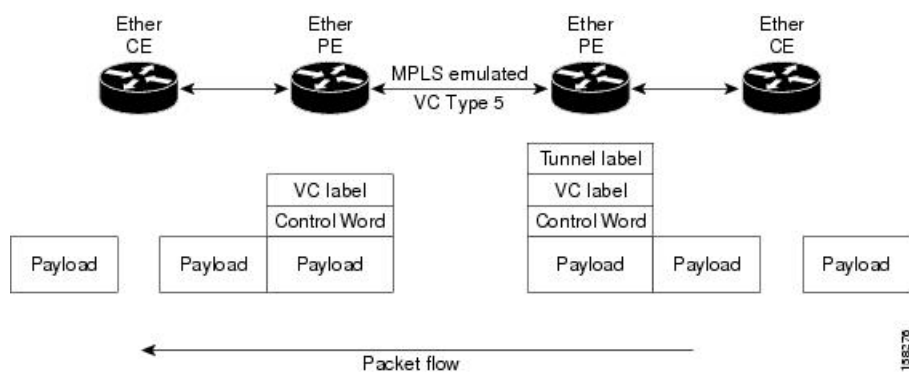
Figure 15: Ethernet Port Mode Packet Flow
