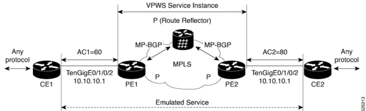
Figure 84: VPWS Traffic flow
