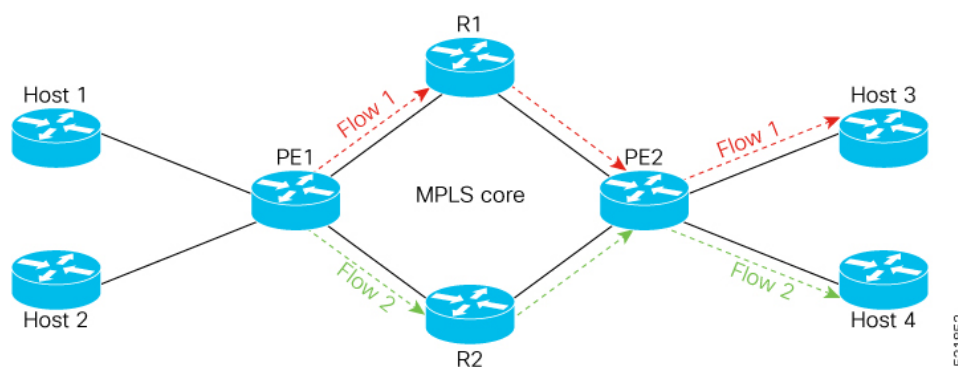
Figure 12: Fat label-based load balancing node workflow
