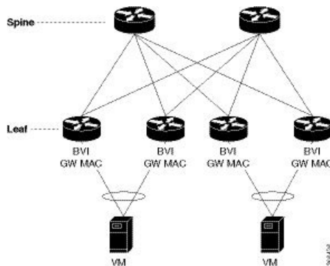
Figure 66: EVPN Multi-Homing All-Active
