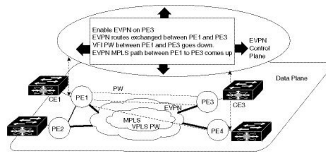
Figure 42: EVPN MPLS Seamless Integration with VPLS
