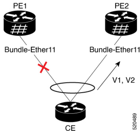
Figure 40: EVPN Port-Active Multihoming
