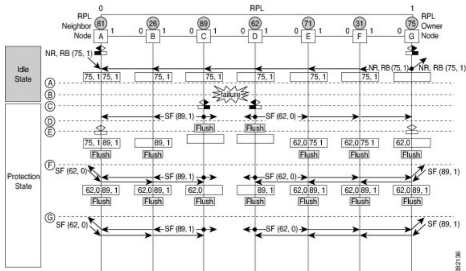
Figure 29: G.8032 Single Link Failure
