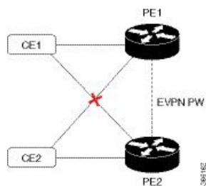
Figure 9: Local Switching
