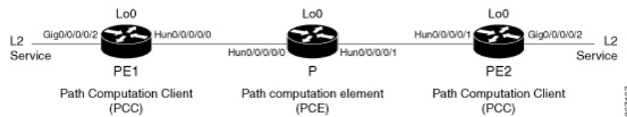
Figure 84: EVPN VPWS On Demand Next Hop with SR-TE
