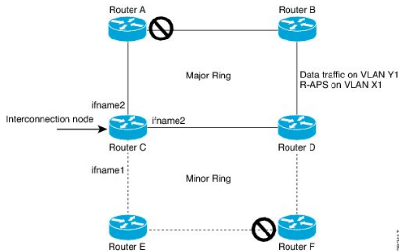
Figure 31: Open Ring Scenario - interconnection node
