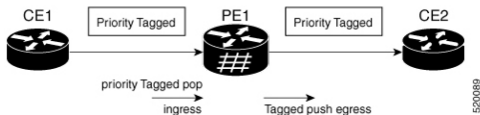
Figure 3: Rewrite of Priority Tag
