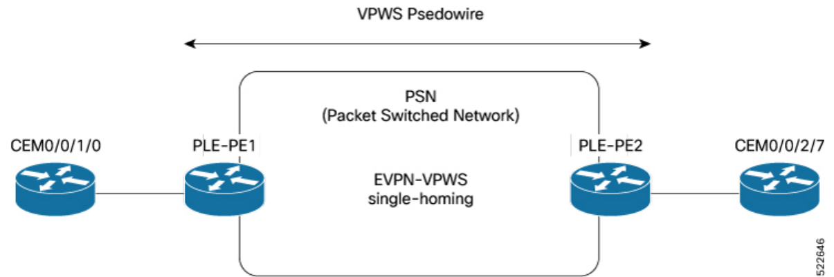
Figure 81: PLE over EVPN VPWS
