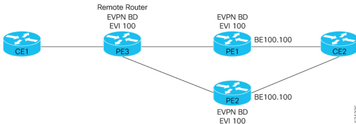
Figure 54: Layer 2 FRR multi-homing topology
