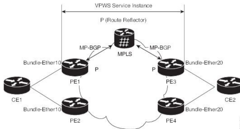
Figure 76: EVPN VPWS Multi-Homed
