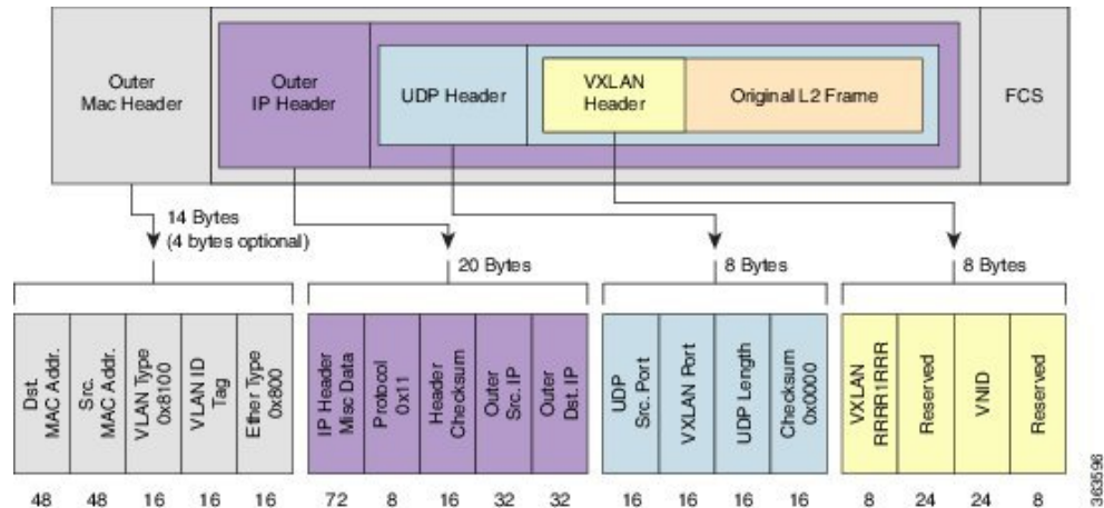
Figure 85: VXLAN Packet Format
