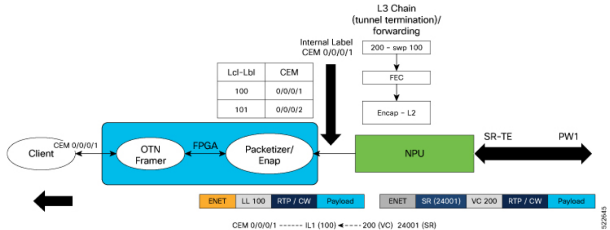
Figure 80: PLE Forwarding Flow – Disposition
