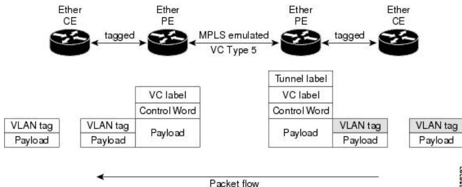
Figure 15: VLAN Mode Packet Flow
