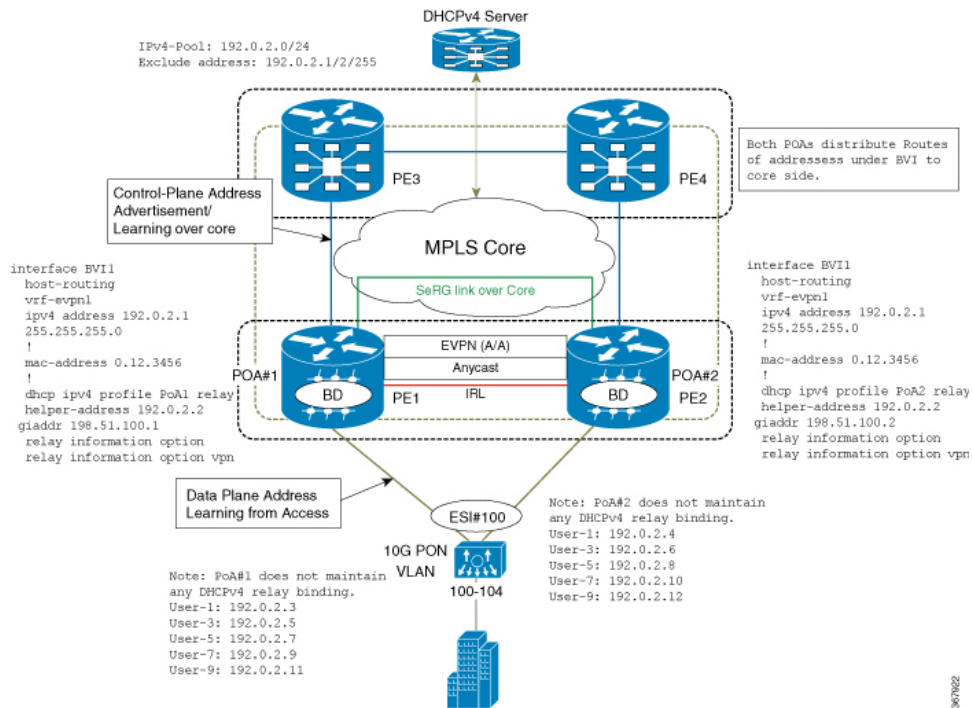
Figure 72: DHCPv4 Relay Handling for EVPN and DHCPv4 Server in Different VRF
