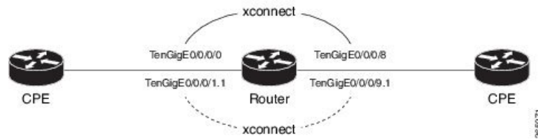
Figure 18: Local Switching Between Attachment Circuits
