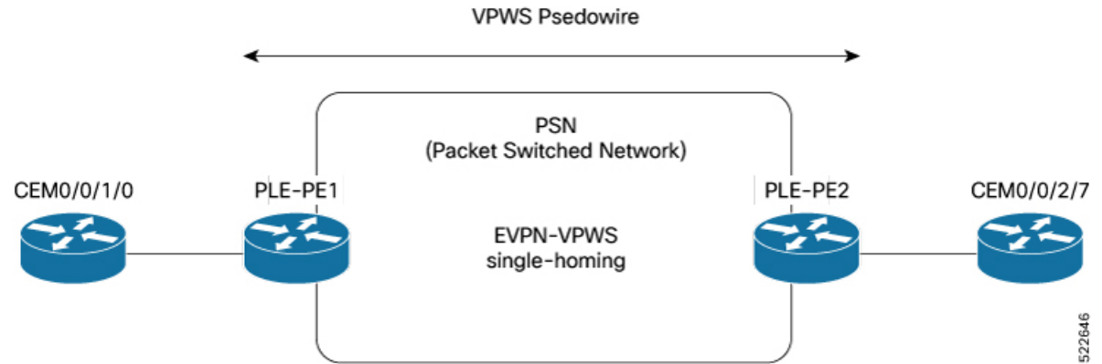
Figure 79: PLE over EVPN VPWS
