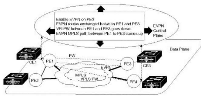
Figure 41: EVPN MPLS Seamless Integration with VPLS
