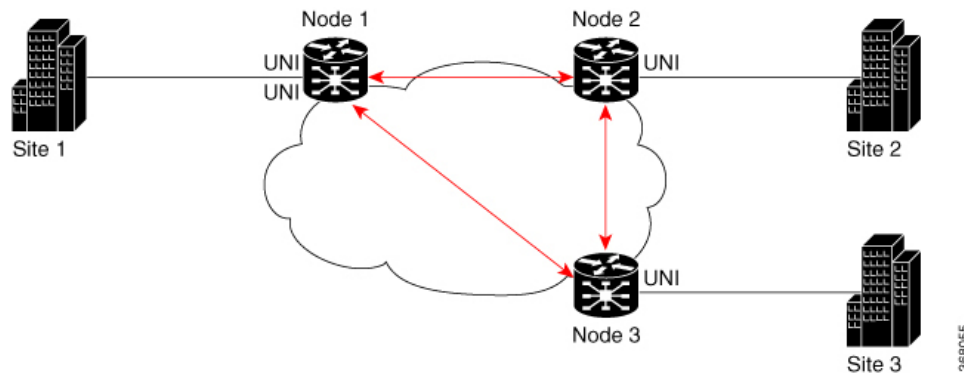
Figure 76: CFM on EVPN VPWS: Full Mesh Topology
