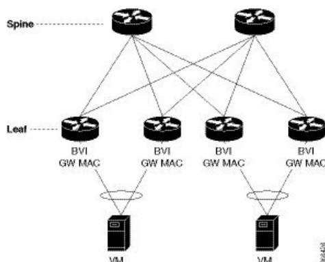
Figure 64: EVPN Multi-Homing All-Active
