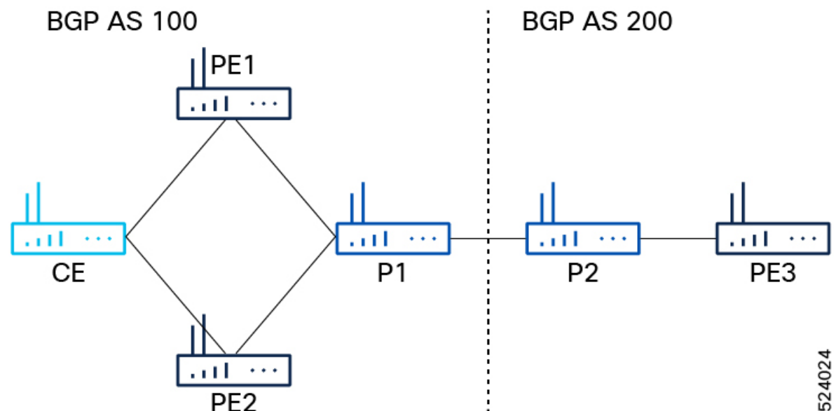
Figure 55: Inter-AS option C
