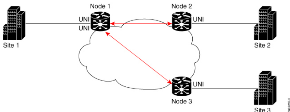
Figure 58: CFM on EVPN ELAN: Hub and Spoke Topology
