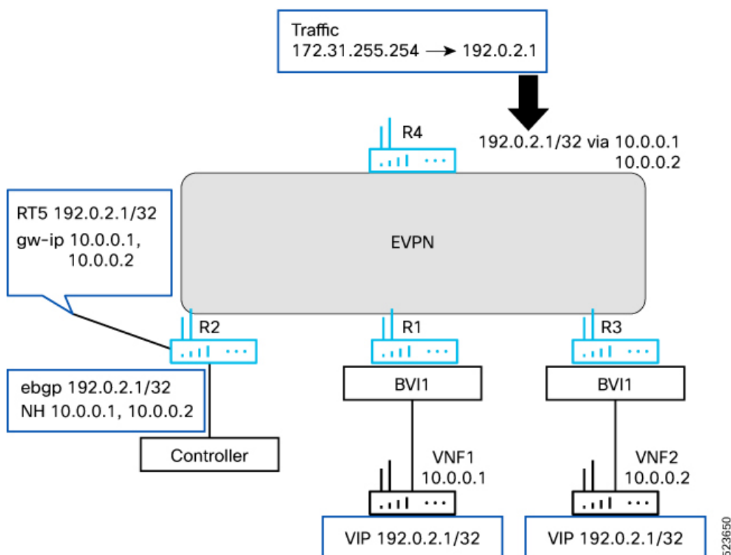
Figure 60: Host-tracking using BFD
