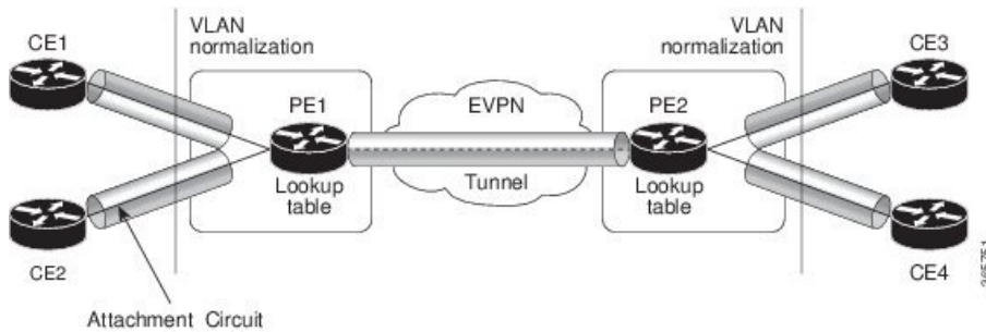
Figure 20: Flexible Cross-Connect Service
