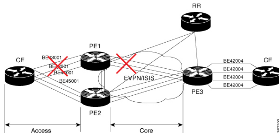
Figure 48: EVPN Core Isolation Protection
