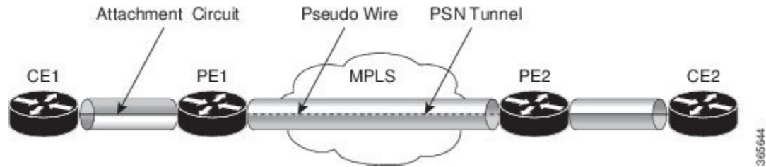
Figure 19: Static Cross-Connect Circuits in a Layer 2 VPN
