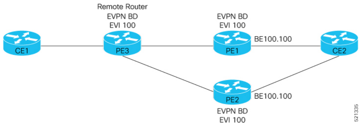
Figure 52: Layer 2 Fast Reroute
