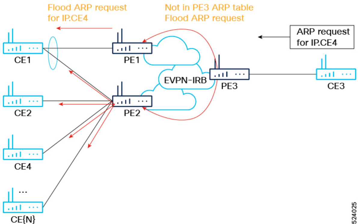
Figure 67: EVPN-IRB Network without ARP and ND Proxy Full Suppression or with ARP Proxy Partial Suppression
