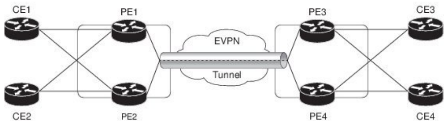
Figure 21: Flexible Cross-Connect Service Multi-Homed
