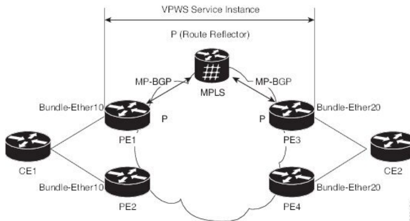
Figure 74: EVPN VPWS Multi-Homed
