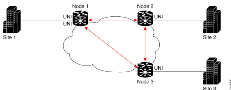
Figure 57: CFM on EVPN ELAN: Full Mesh Topology
