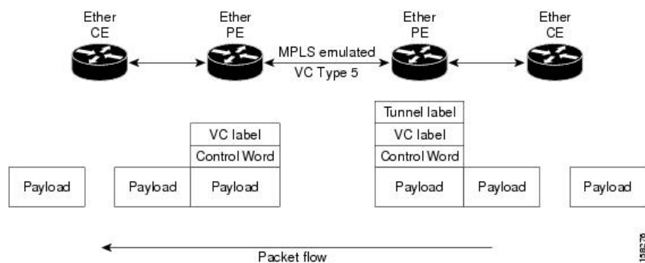
Figure 14: Ethernet Port Mode Packet Flow
