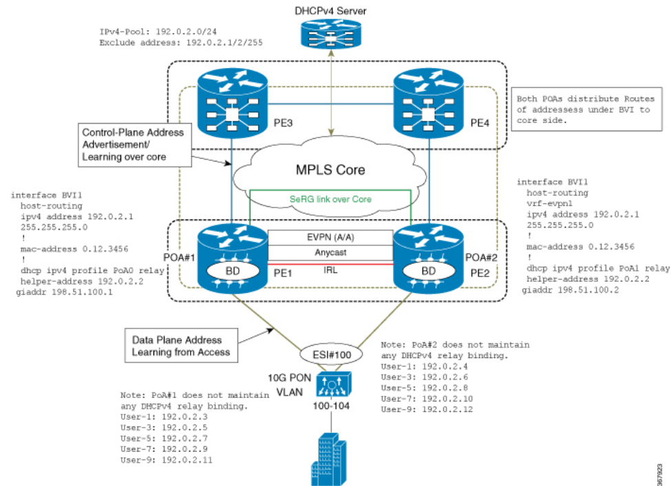
Figure 71: DHCPv4 Relay Handling for EVPN and DHCPv4 Server in Default VRF
