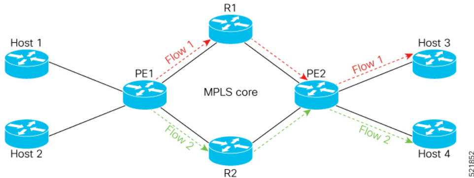
Figure 12: Fat label-based load balancing on L2VPN decapsulation node workflow
