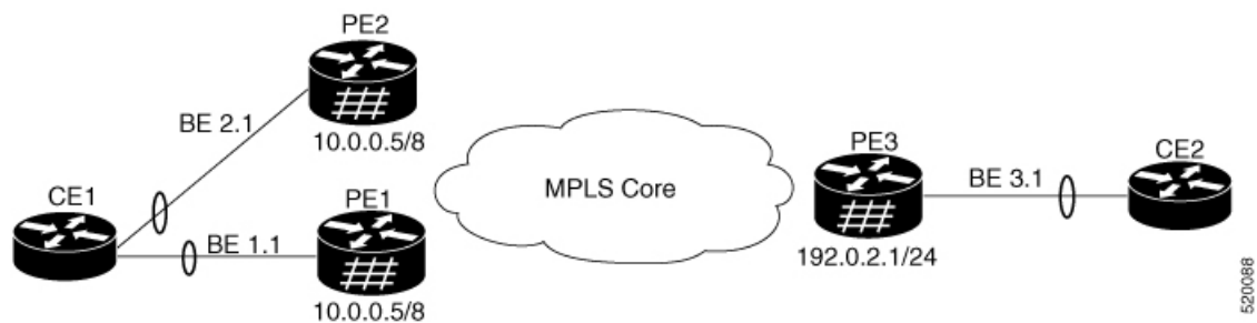
Figure 65: EVPN: Single-Active Multihoming for Anycast Gateway IRB
