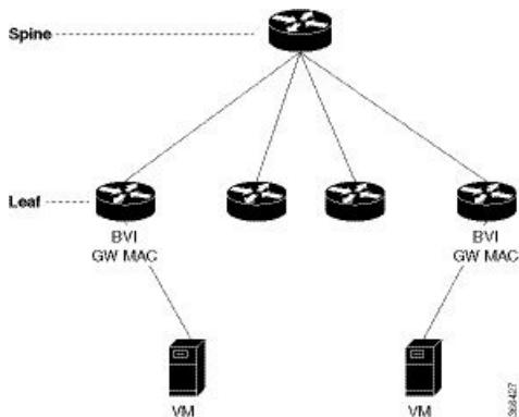
Figure 63: EVPN Single-Homing Access Gateway
