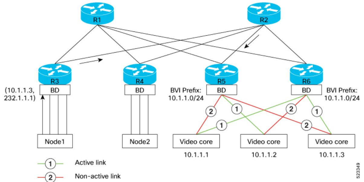
Figure 66: Traffic Flow from Video Core to Node
