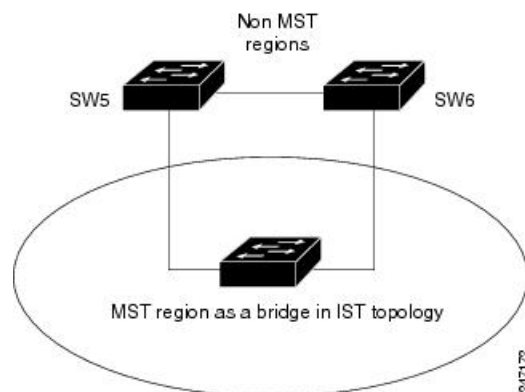
Figure 37: Logical Topology in MST Region Interacting with Non-MST Bridges
