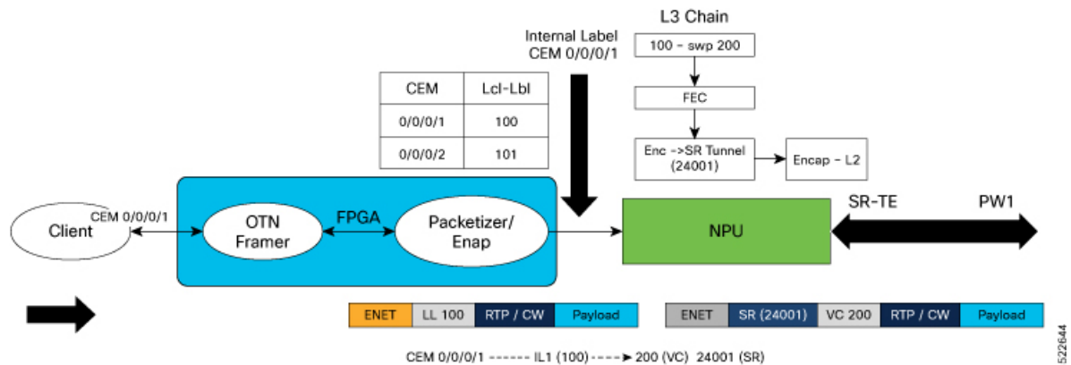
Figure 77: PLE Forwarding Flow – Imposition
