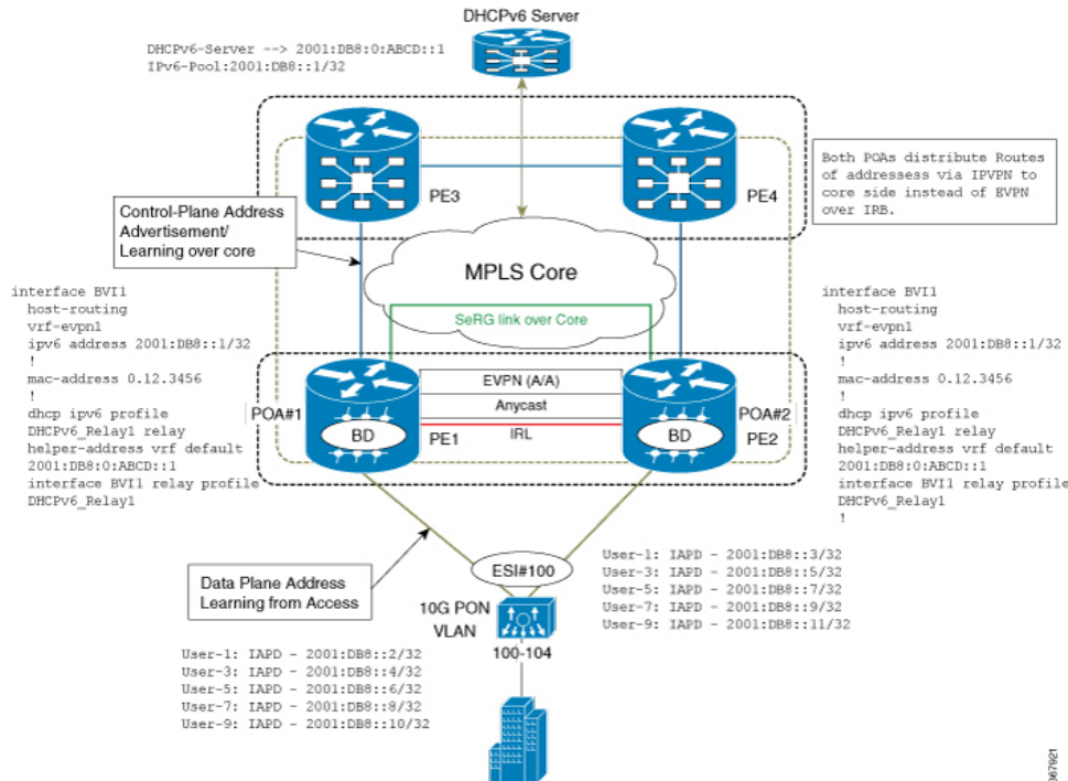
Figure 73: DHCPv6 relay Handling for EVPN and DHCPv6 Server in Default VRF
