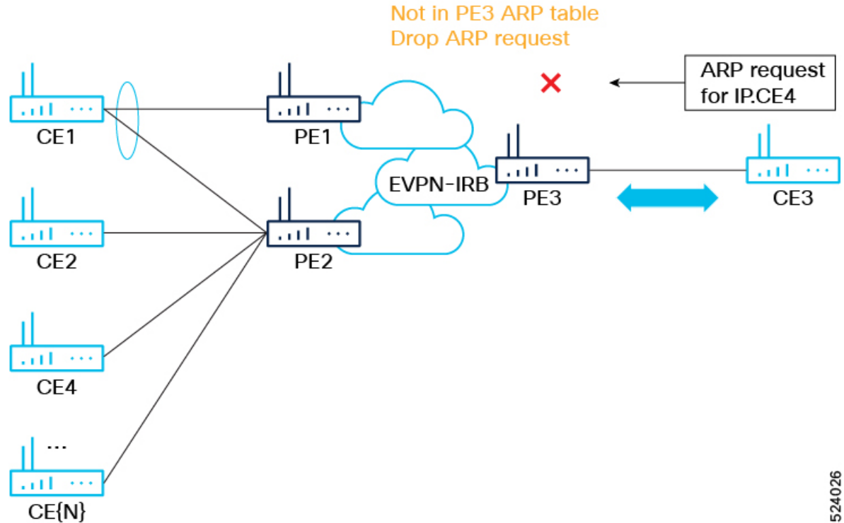
Figure 68: EVPN-IRB Network with ARP and ND Proxy Full Suppression
