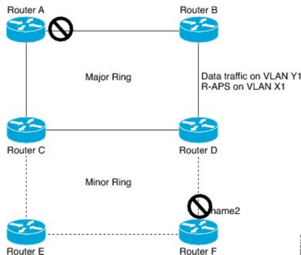
Figure 31: Open Ring Scenario
