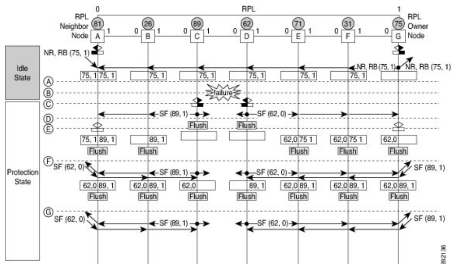
Figure 28: G.8032 Single Link Failure
