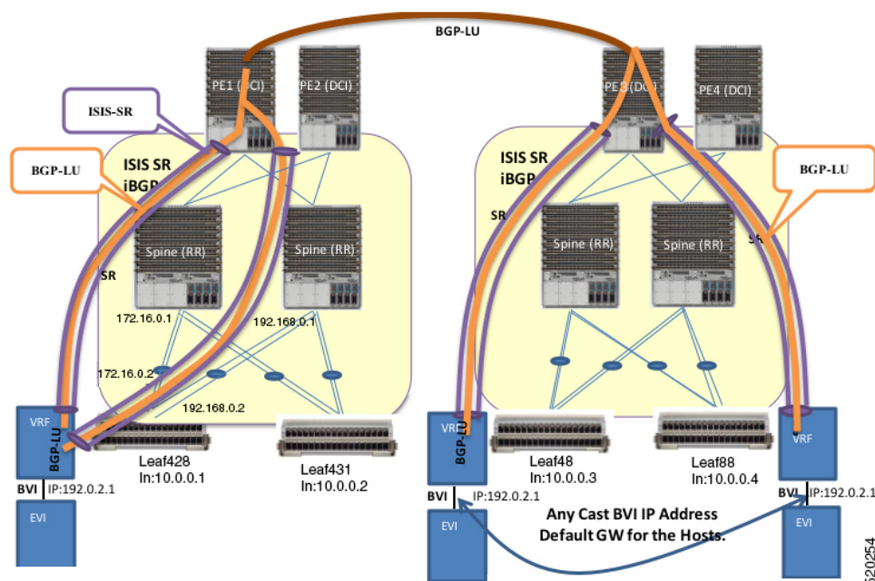
Figure 51: EVPN Bridging and VPWS Services over BGP-LU Underlay
