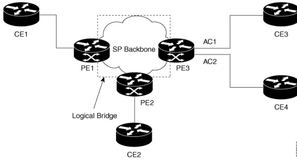
Figure 26: Split Horizon Group 2
