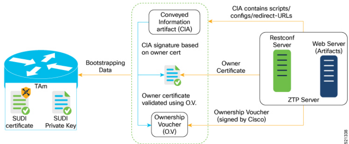
Figure 3: Server Validation
