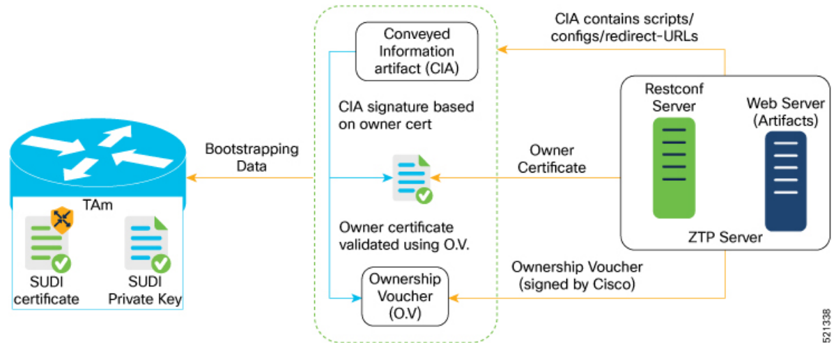
Figure 3: Server Validation
