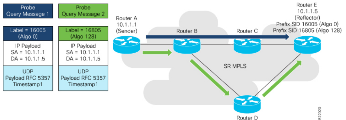
Figure 35: Delay Measurement Probe Toward an IP Endpoint Using Custom Labeled Paths
