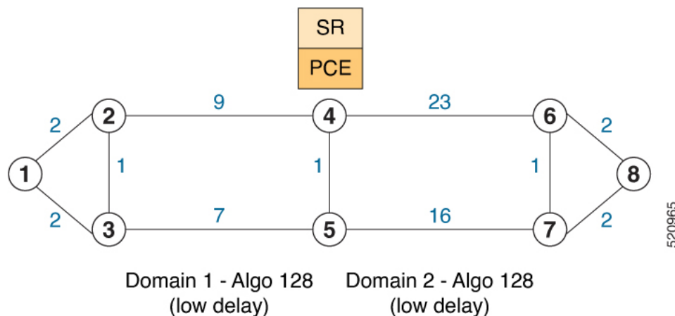
Figure 28: Multi-Domain Topology
