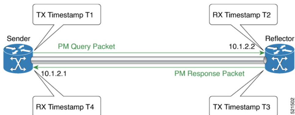
Figure 31: Two-Way
