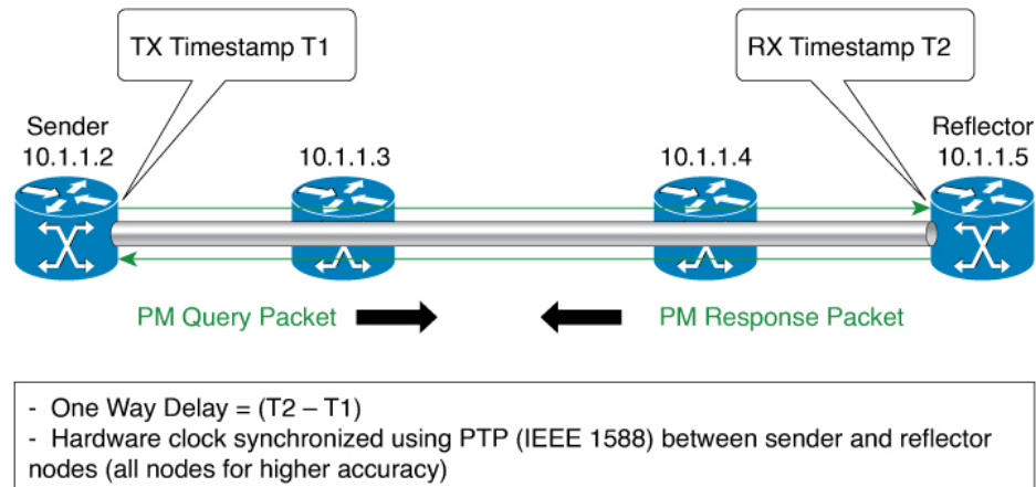
Figure 30: One-Way
