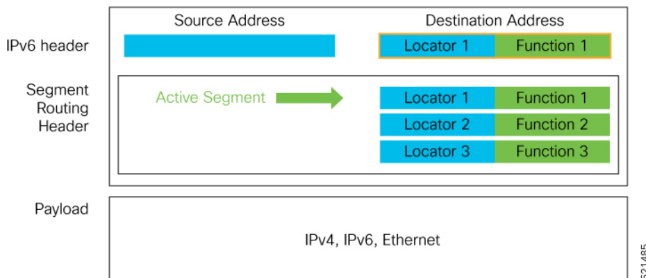
Figure 10: Network Program in the Packet Header
