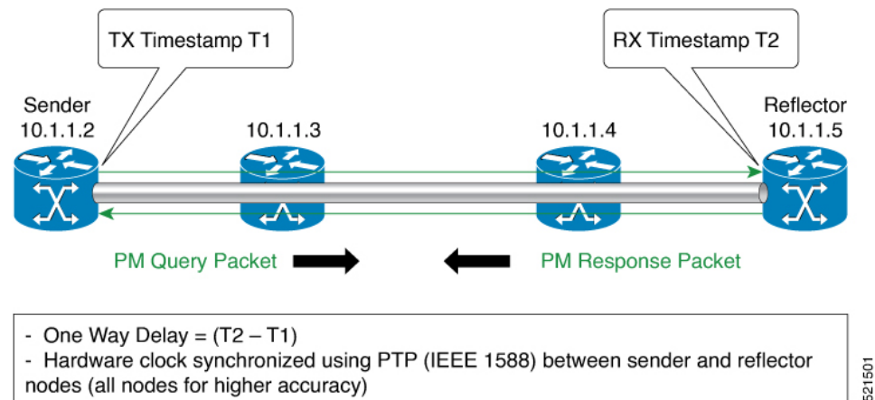
Figure 30: One-Way
