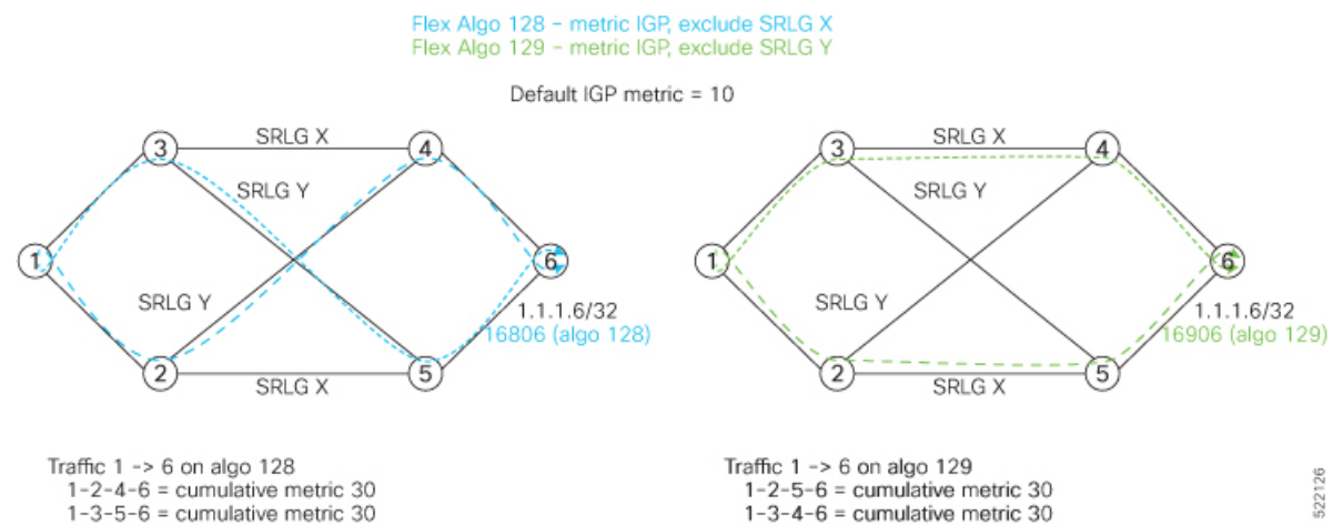
Figure 27: Flex Algo with Exclude SRLG Constraint
