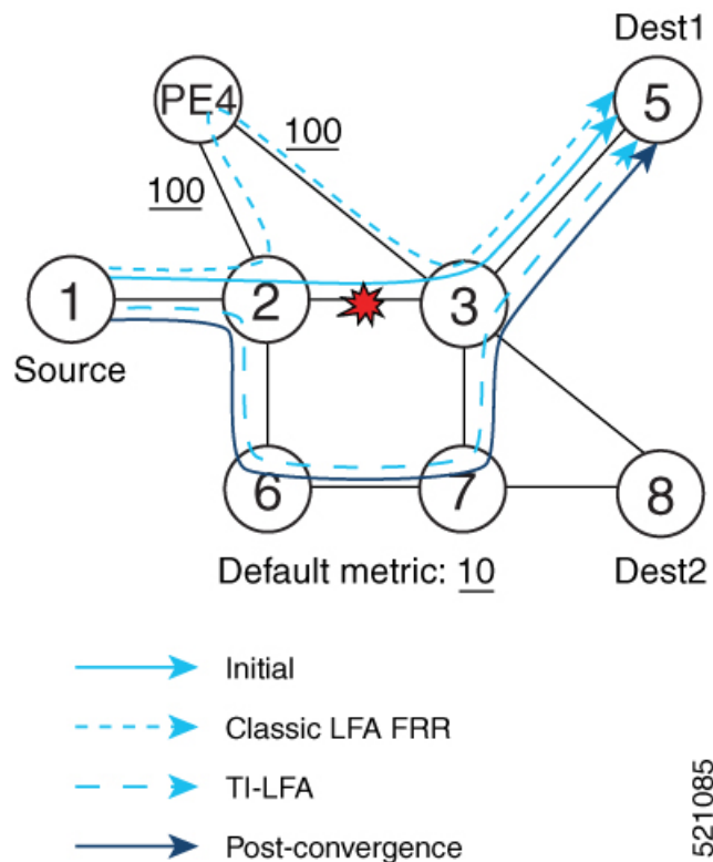
Figure 37: TI-LFA Repair Path
