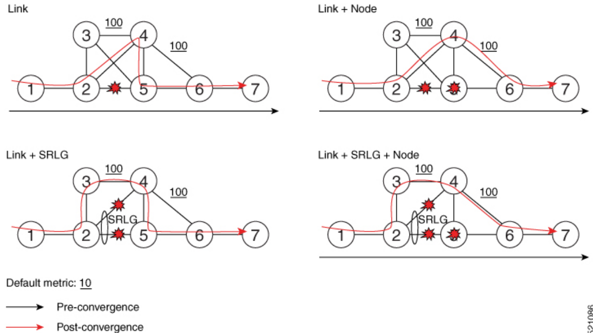
Figure 38: TI-LFA Protection Types
