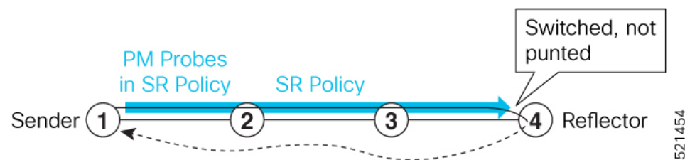
Figure 32: Loopback
