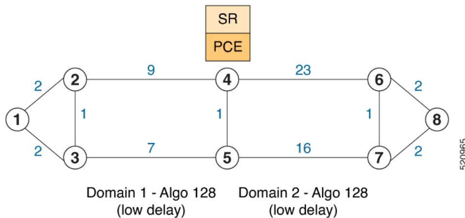
Figure 28: Multi-Domain Topology
