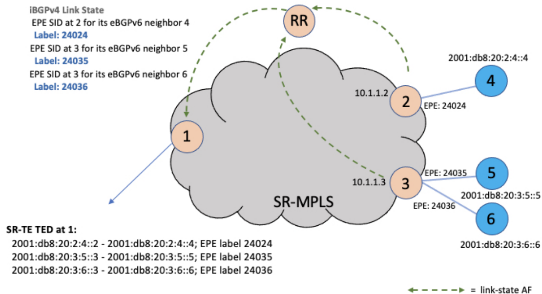
Figure 20: BGP-LS
