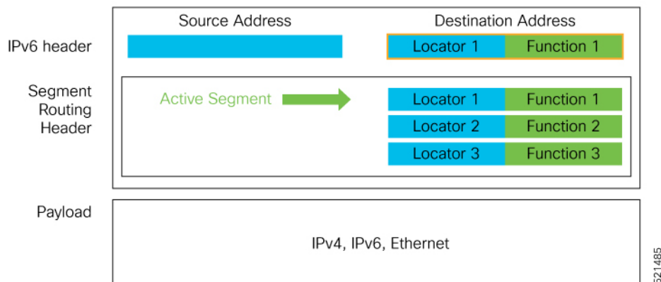
Figure 10: Network Program in the Packet Header
