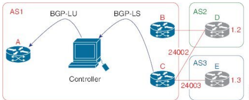
Figure 15: Topology
