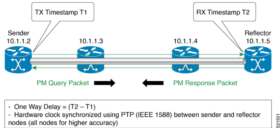
Figure 41: One-Way
