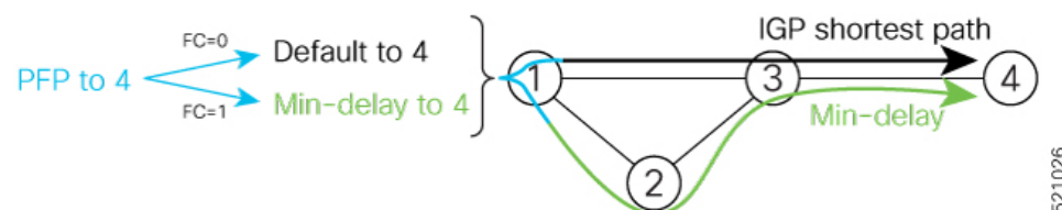
Figure 18: PFP Example
