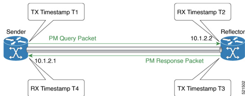
Figure 42: Two-Way
