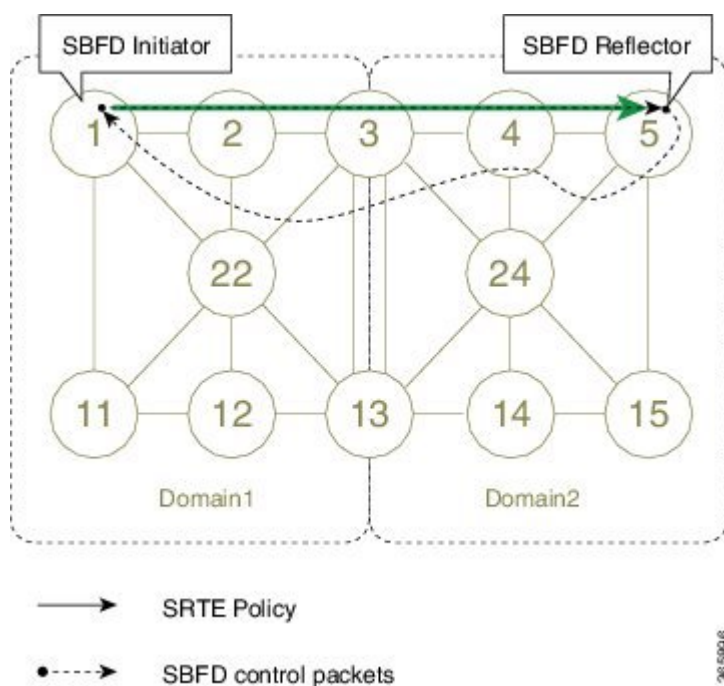
Figure 8: S-BFD Initiator and Reflector
