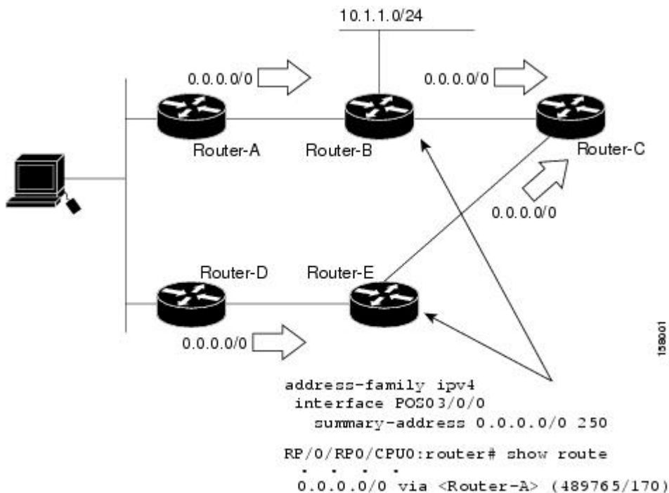
Figure 14: Floating Summary Route Applied for Dual-Homed Remotes
