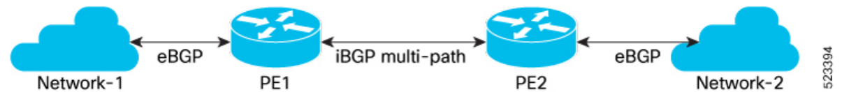
Figure 10: Sample Topology (iBGP)
