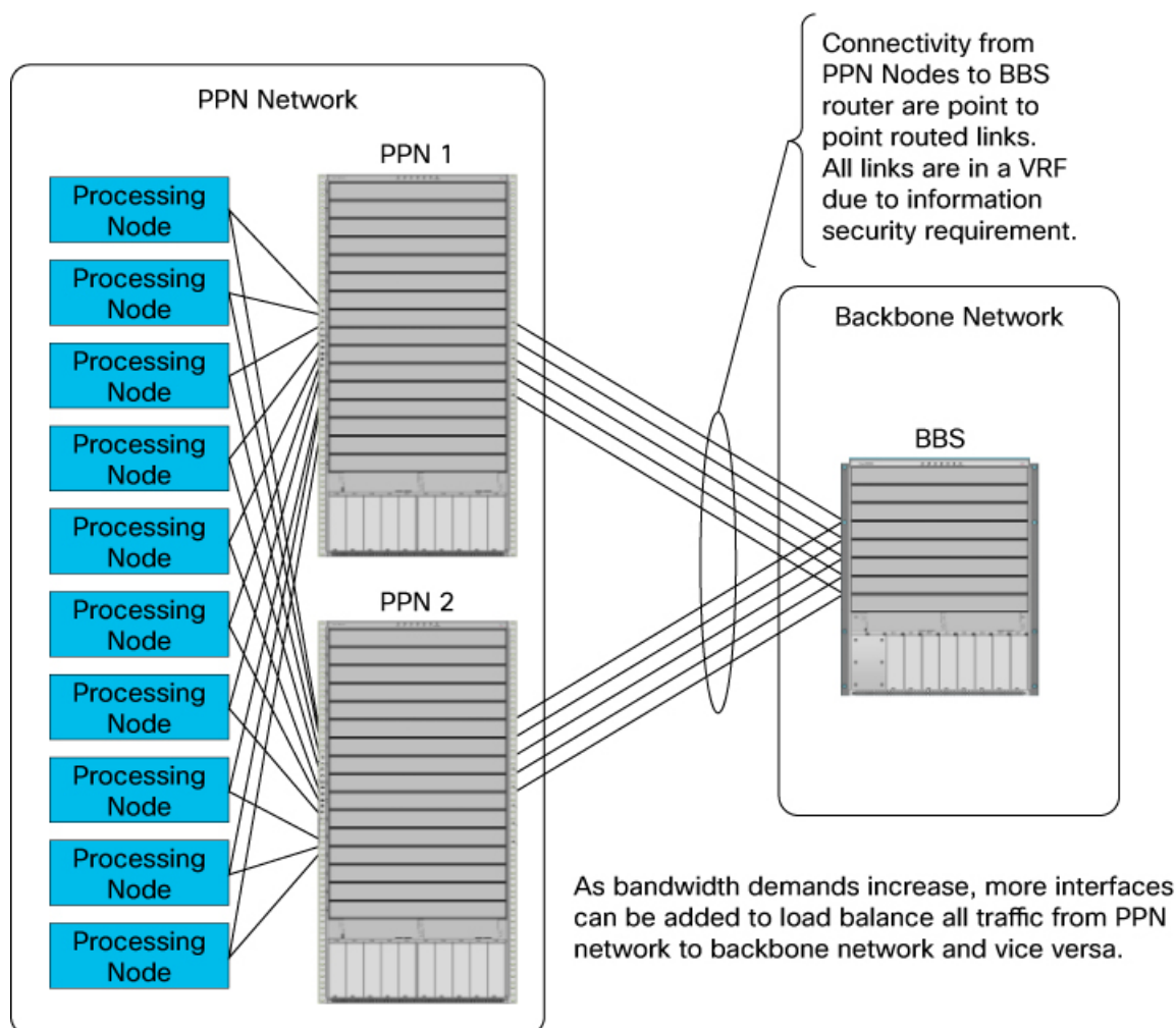
Figure 11: Sample Topology with VRF Links
