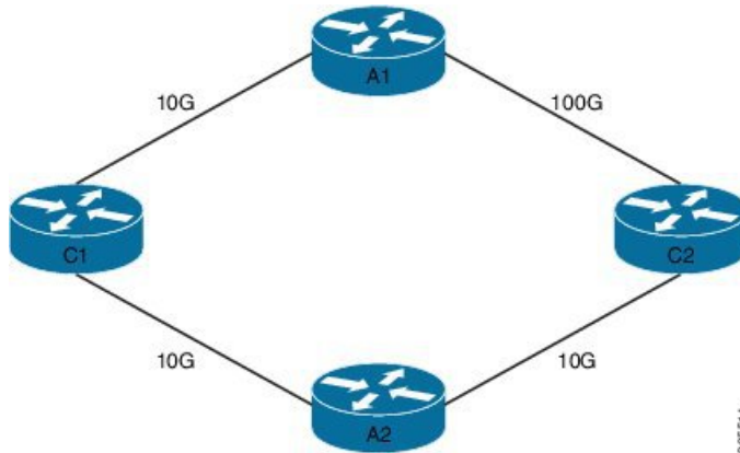
Figure 7: Unequal Cost Multipath for Static Routing
