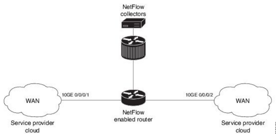
Figure 1: SP-PE Topology
