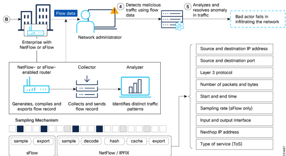
Figure 2: Traffic monitoring workflow with Flow data to identify malicious activity
