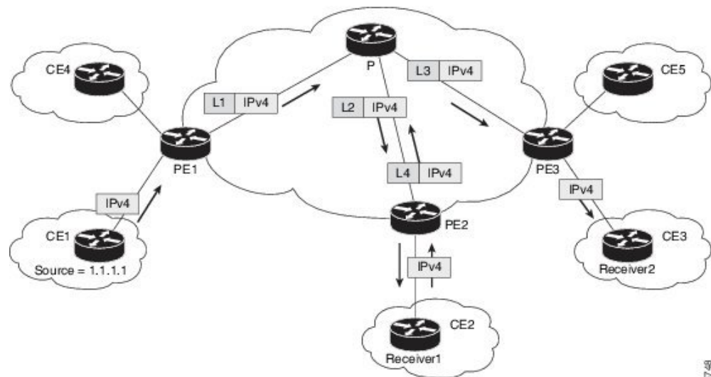
Figure 5: MLDP based MPLS Network for Core and Edge Routers
