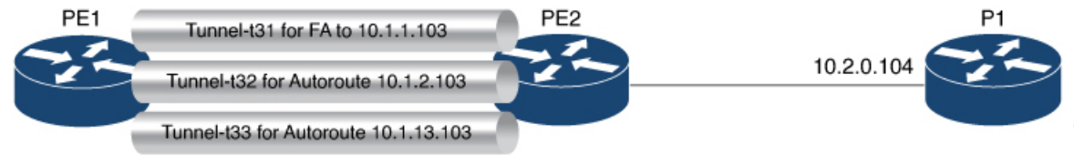
Figure 14: Topology
