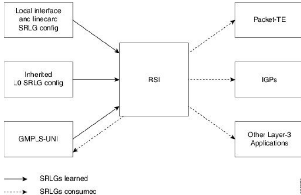
Figure 2: SRLG Communication
