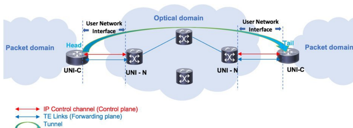
Figure 20: GMPLS UNI
