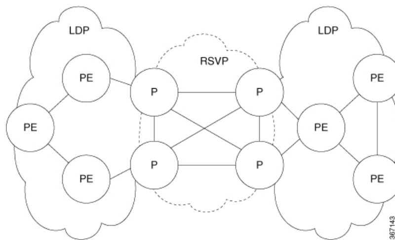
Figure 3: LDP over MPLS-TE
