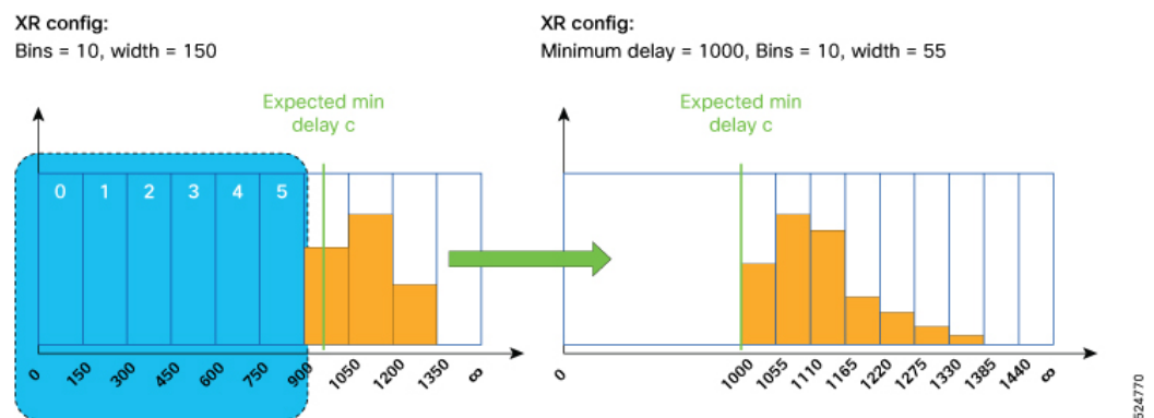
Figure 12: Comparison diagram before and after minimum-delay configuration
