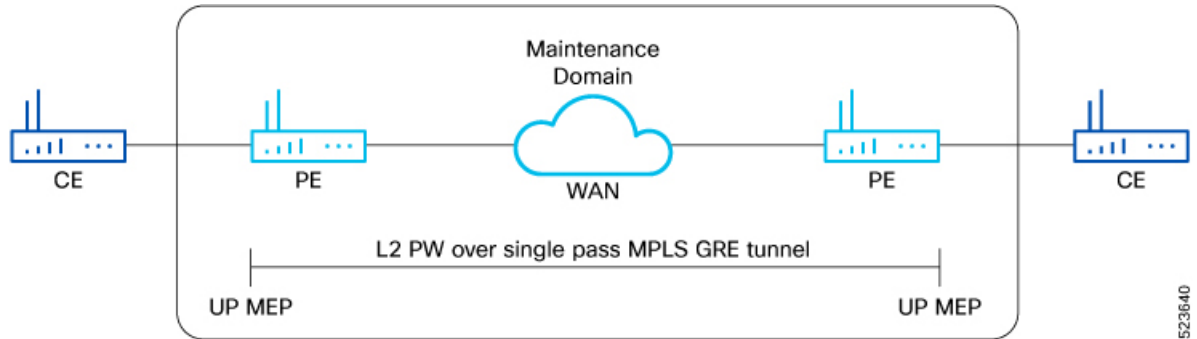
Figure 9: Sample Topology
