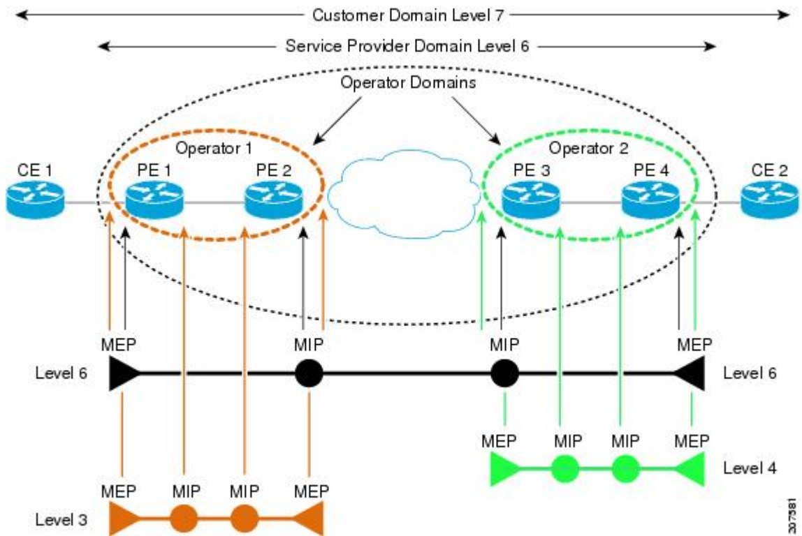
Figure 10: Different CFM Maintenance Domains Across a Network
