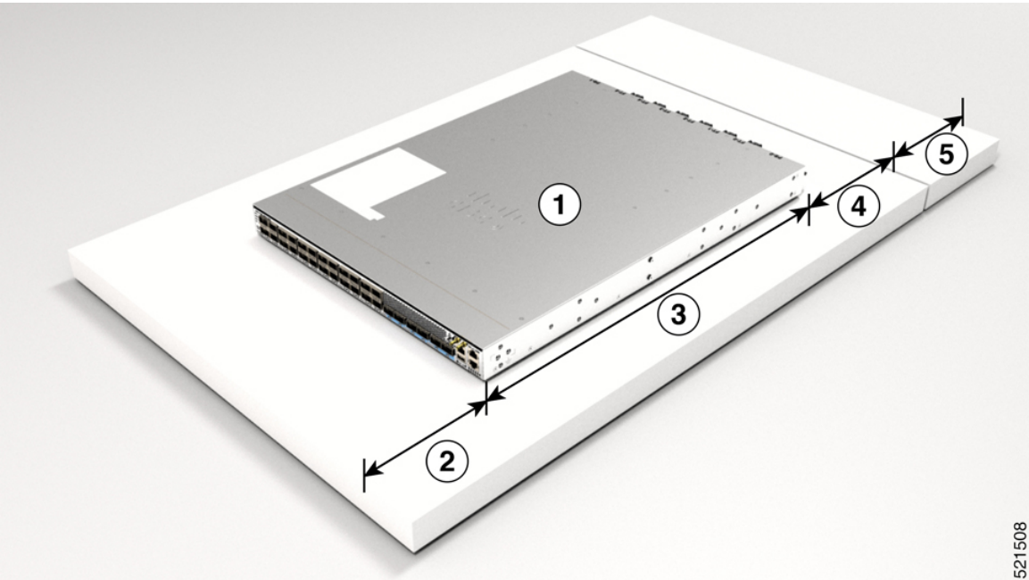
Figure 2: Clearance Requirement
